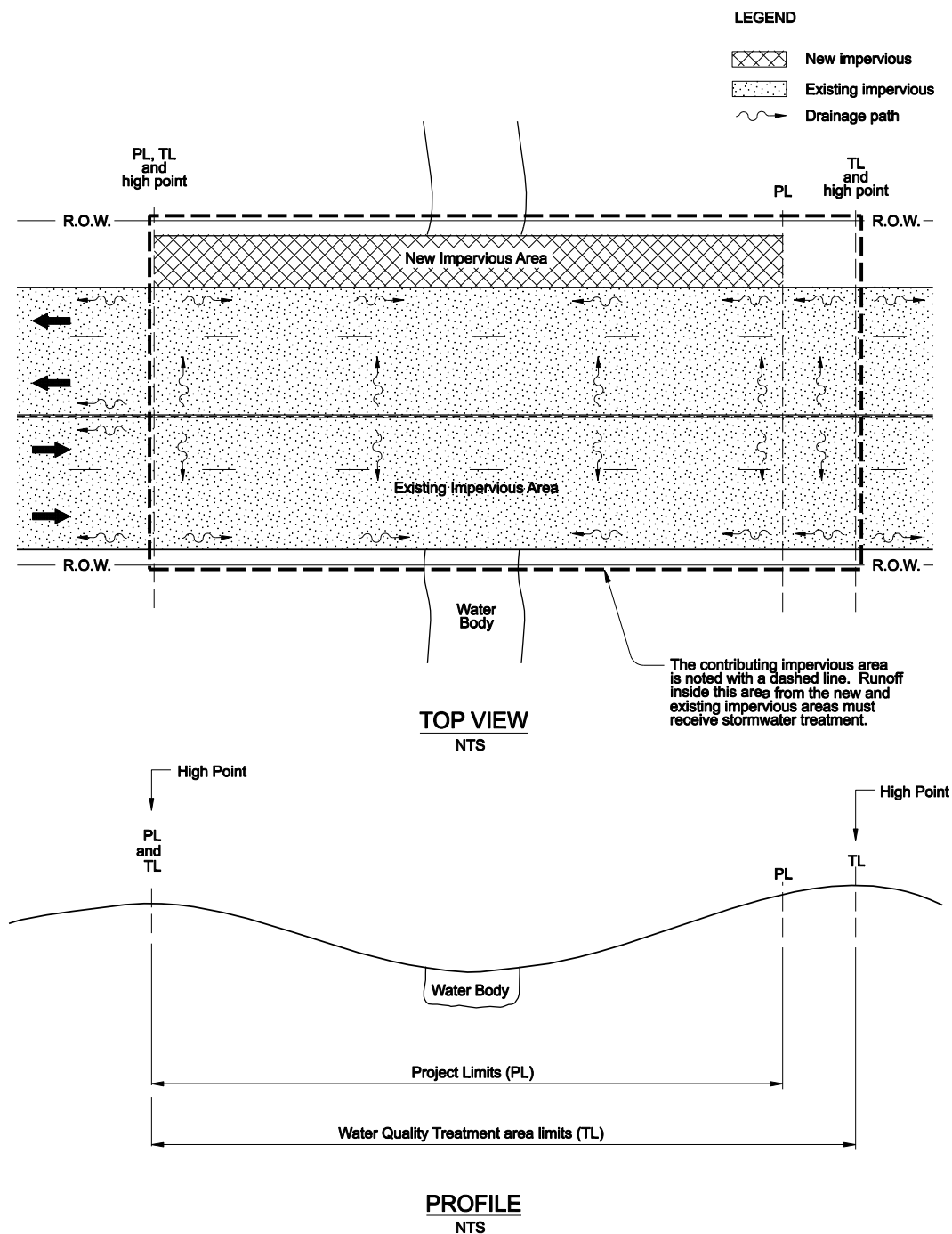
Figure 14-3 Treatment Area Limits (ODOT Transportation project example)
