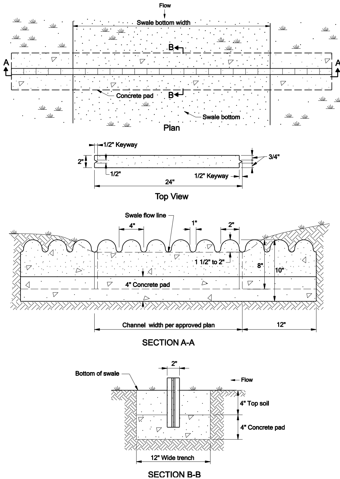
Figure 8 Anchored Concrete Flow Spreader
