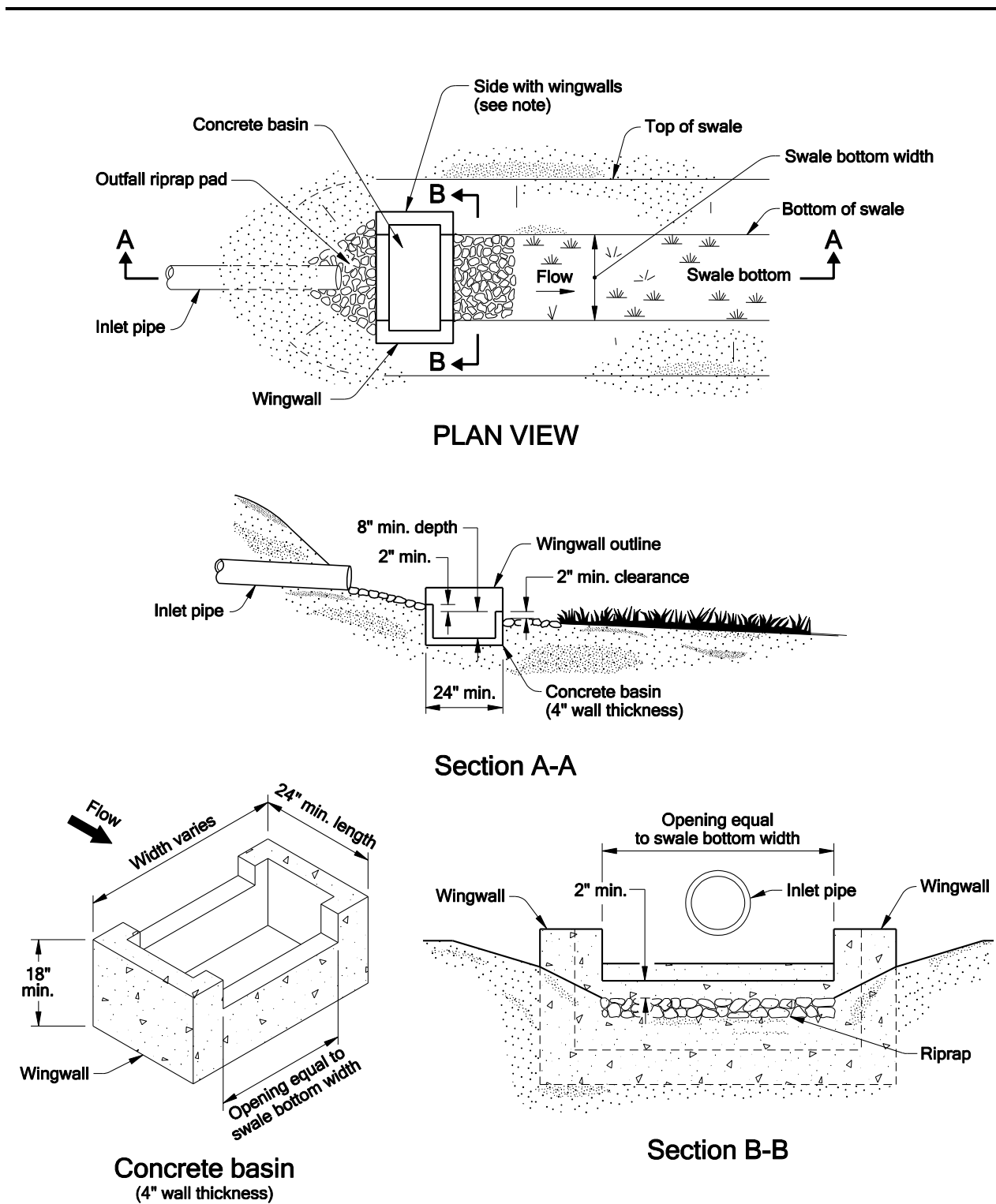
Figure 5 Concrete Basin Flow Spreader
