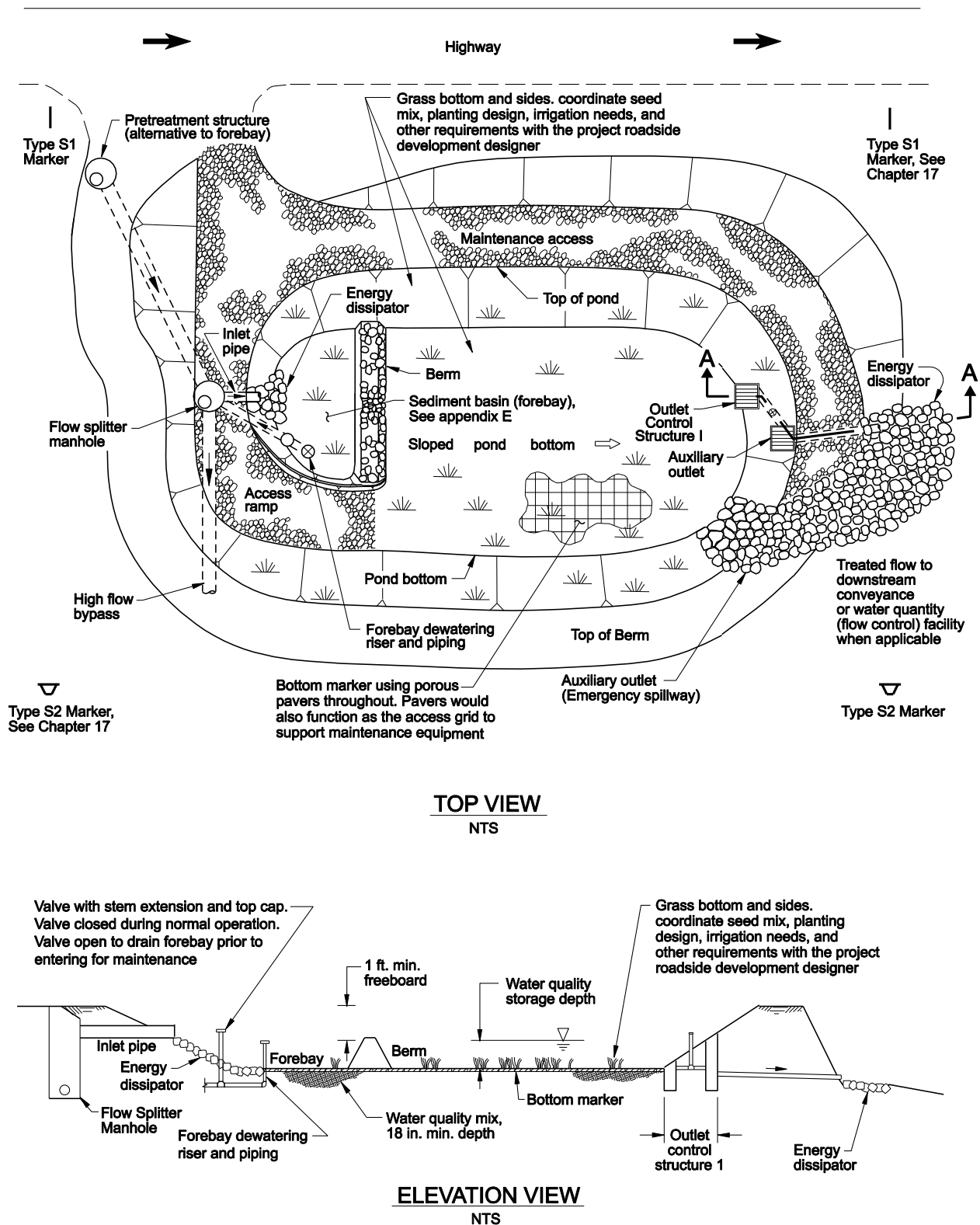
Figure 2 Extended Detention Dry Pond
