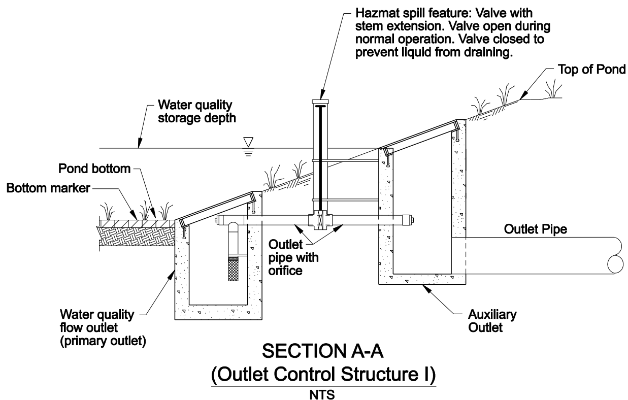
Figure 3 Extended Detention Dry Pond Outlet Control Structure
