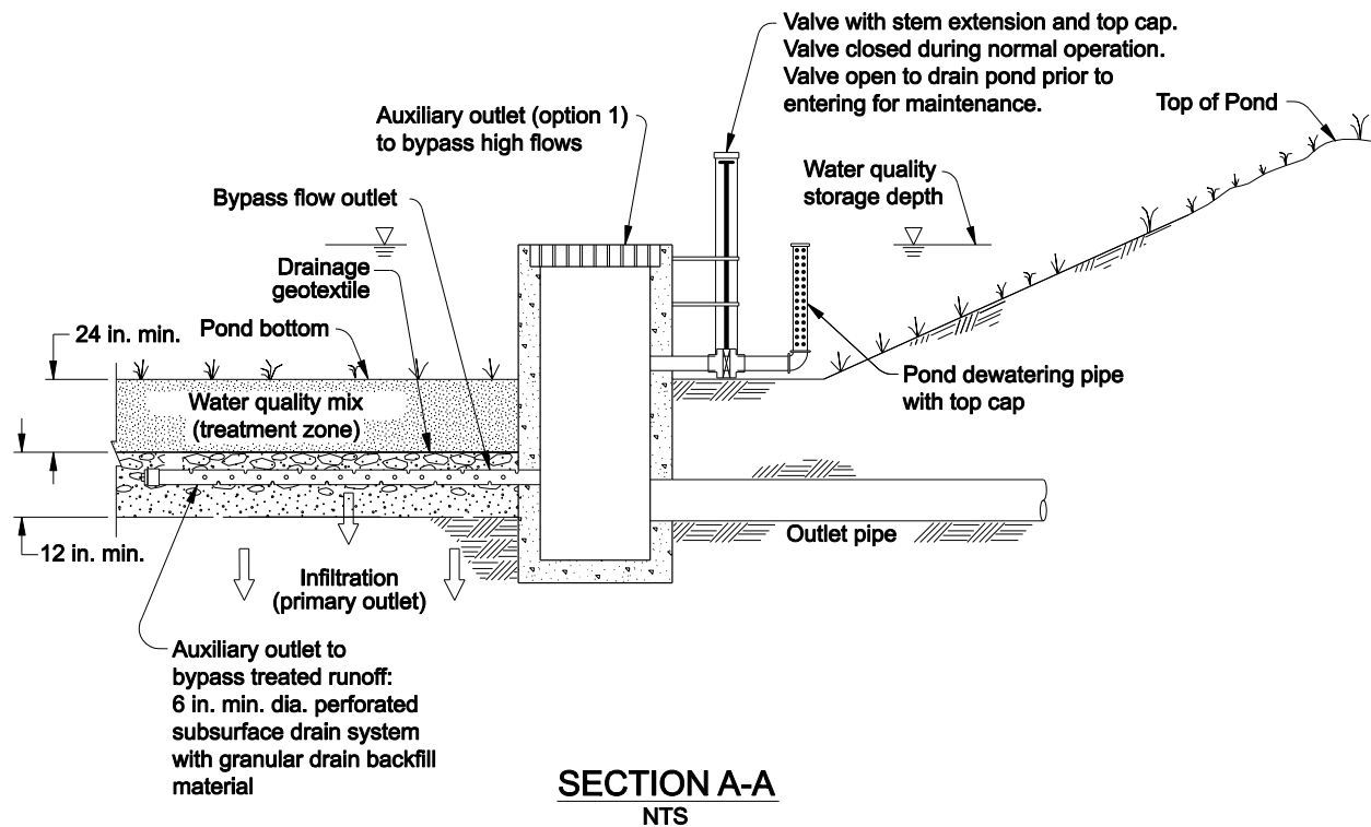
(Cross-Section using a perforated subsurface drain system)
