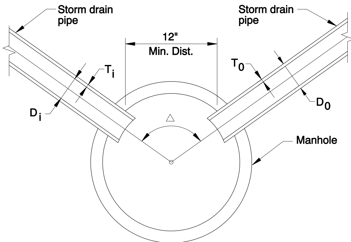
Figure 1 Manhole Sizing
