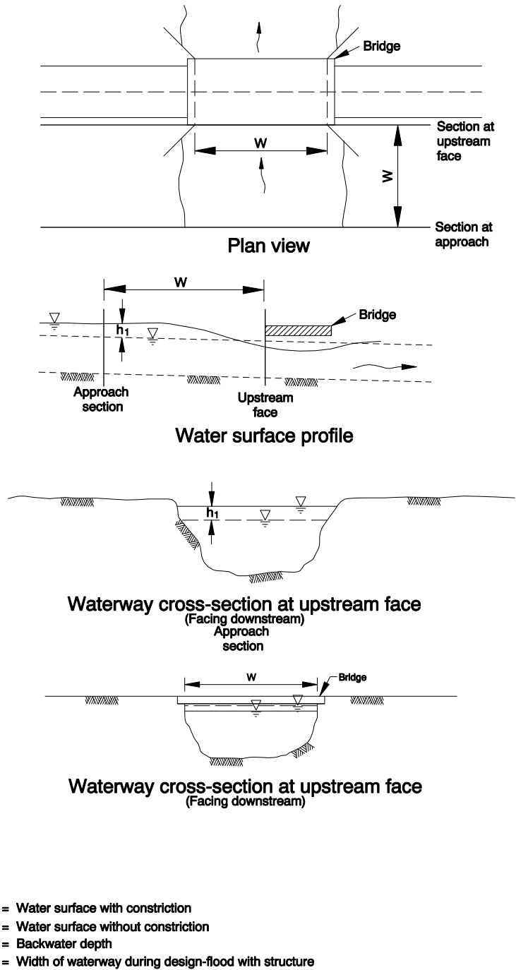
Figure 10-13 Backwater
