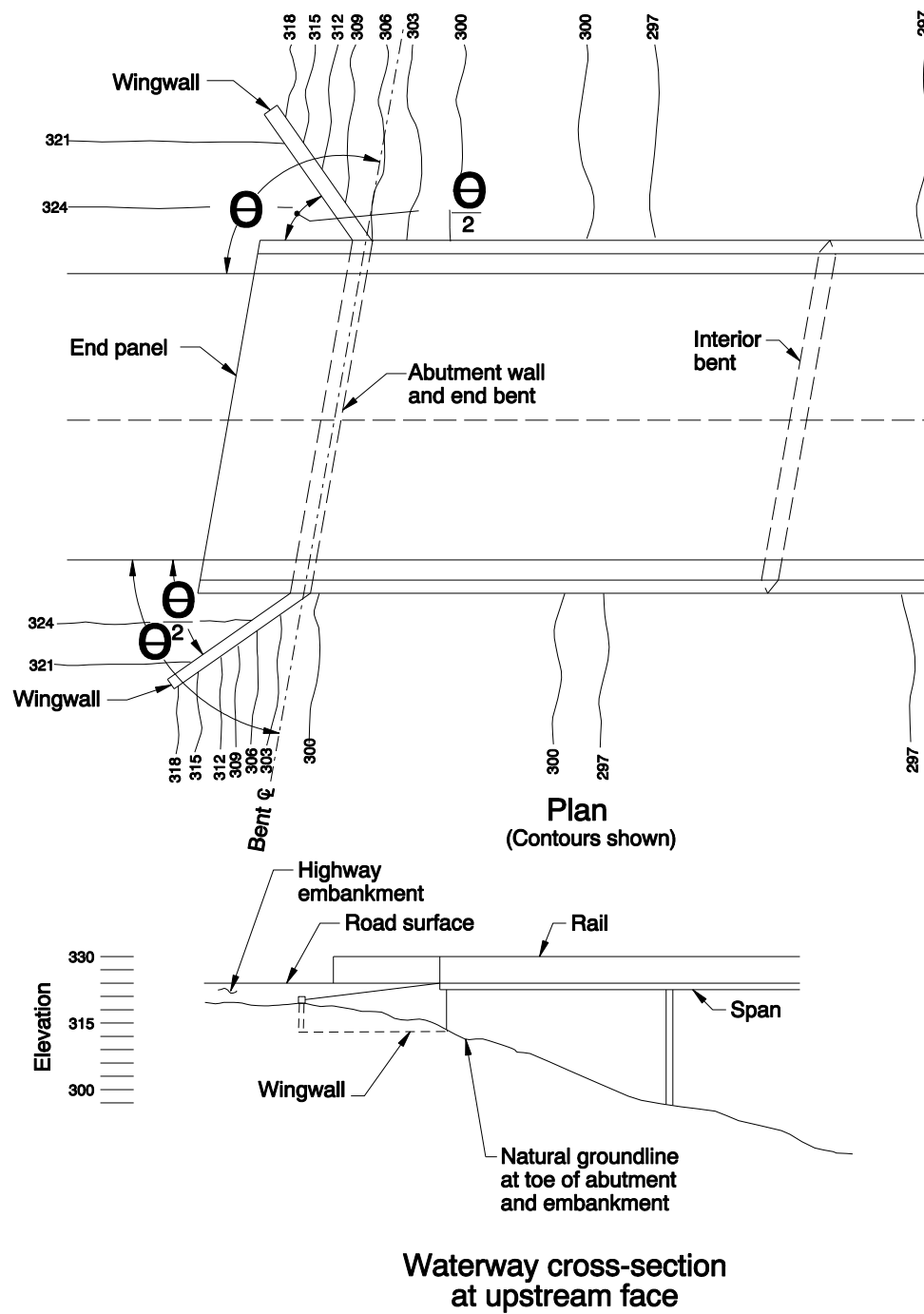
Figure 10-9 Vertical Abutment
