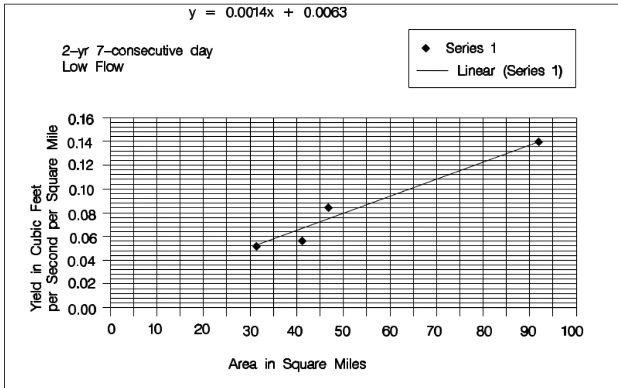
Figure 1 2-Year 7-Consecutive Day Low Flow Relationship for Basins near Miner Creek
