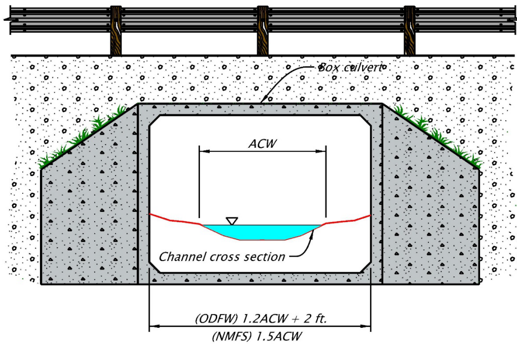
Figure 9 - 10 Box culvert
