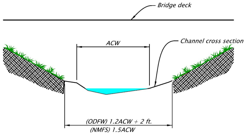
Figure 9 - 12 Bridge width
