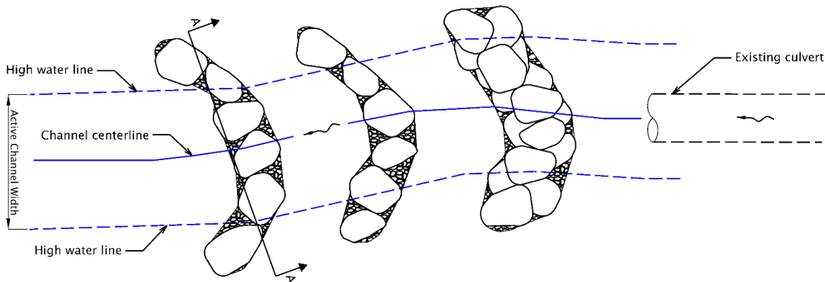
Figure 9 - 17 Step Pool plan view
