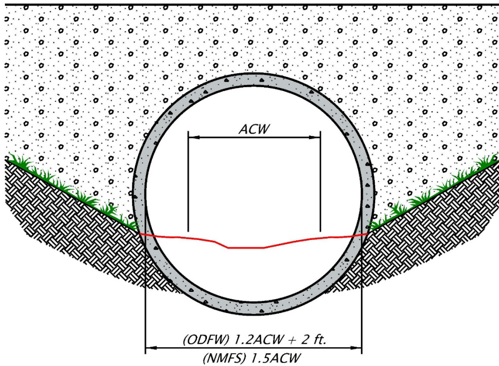
Figure 9 - 9 Circular culvert
