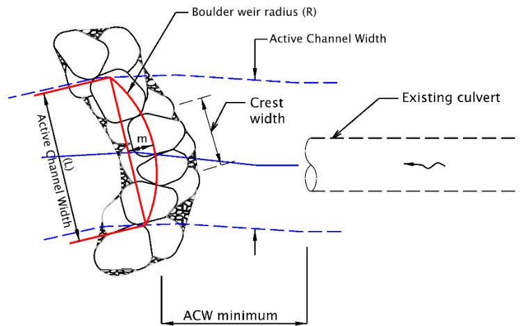
Figure 9 - 14 Boulder Weir plan view
