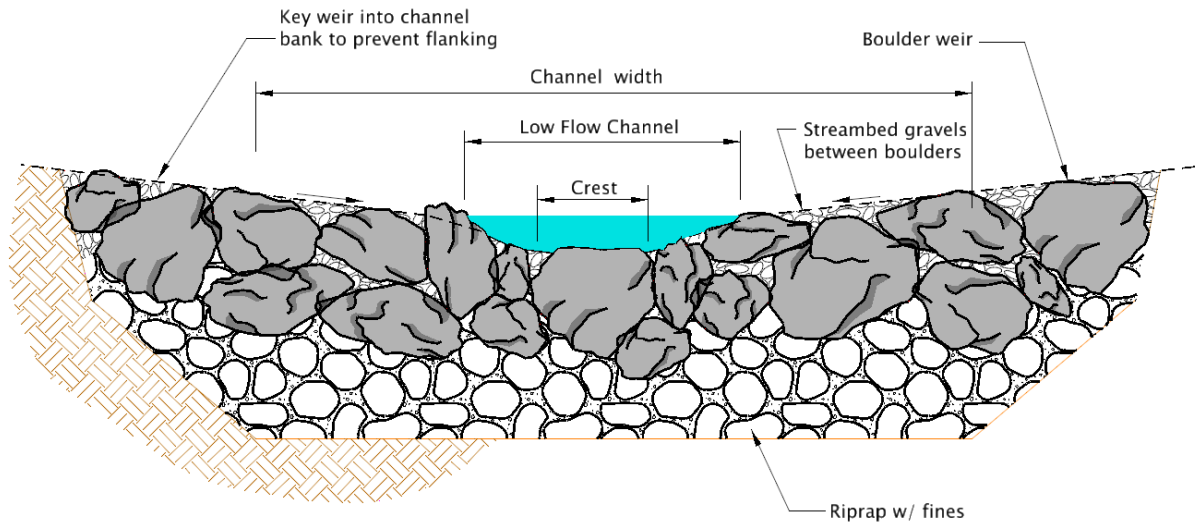
Figure 9 - 16 Boulder Weir cross section
