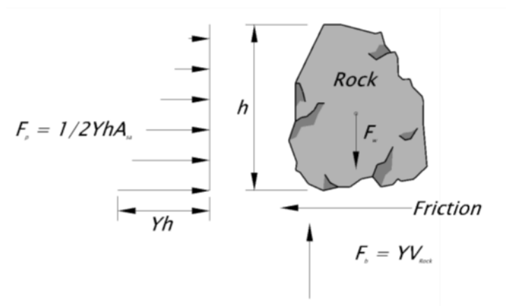
Figure 9 - 13 Rock free body diagram
