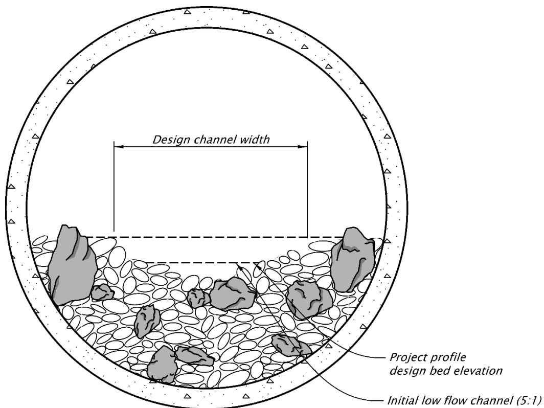
Figure 9 - 7 Channel section within culvert
