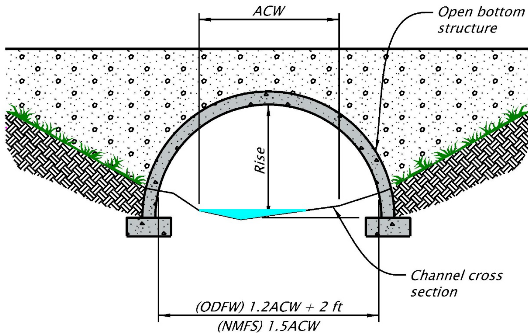
Figure 9 - 11 Open bottom structure
