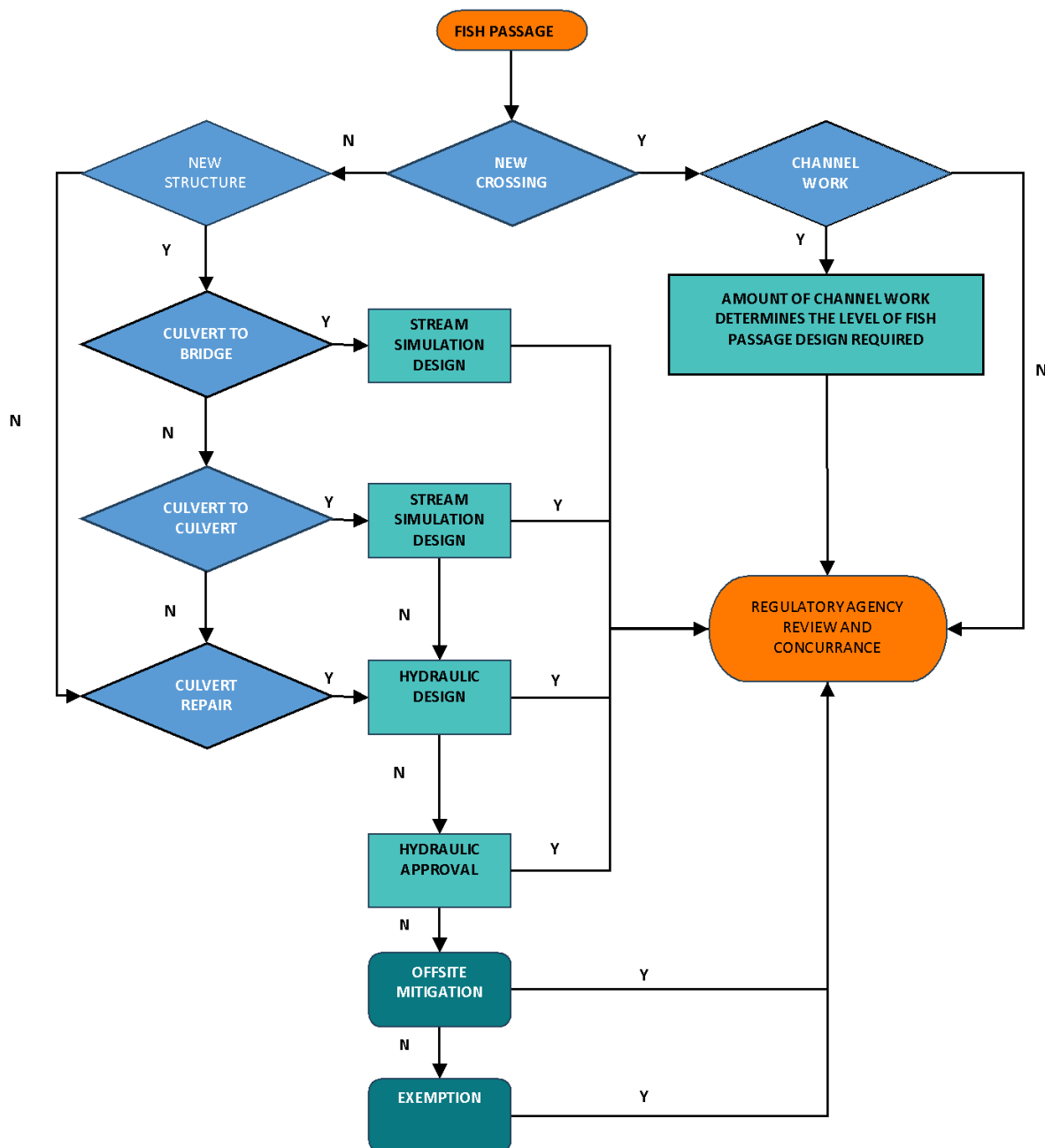
Figure 9 - 1 Fish Passage Project Flow Chart
