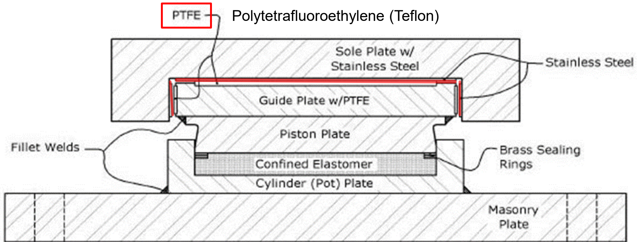
GUIDED EXPANSION POT BEARING
