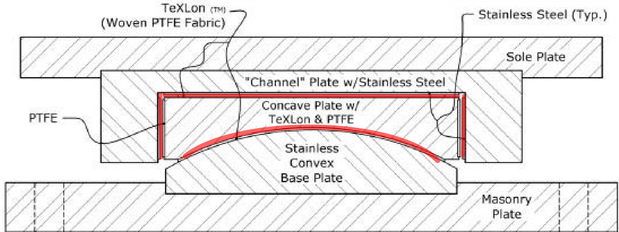
GUIDED EXPANSION SPHERICAL BEARING
