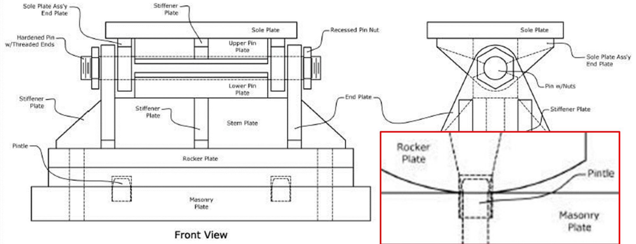
EXPANSION "ROCKER" BEARING - PIN STYLE
