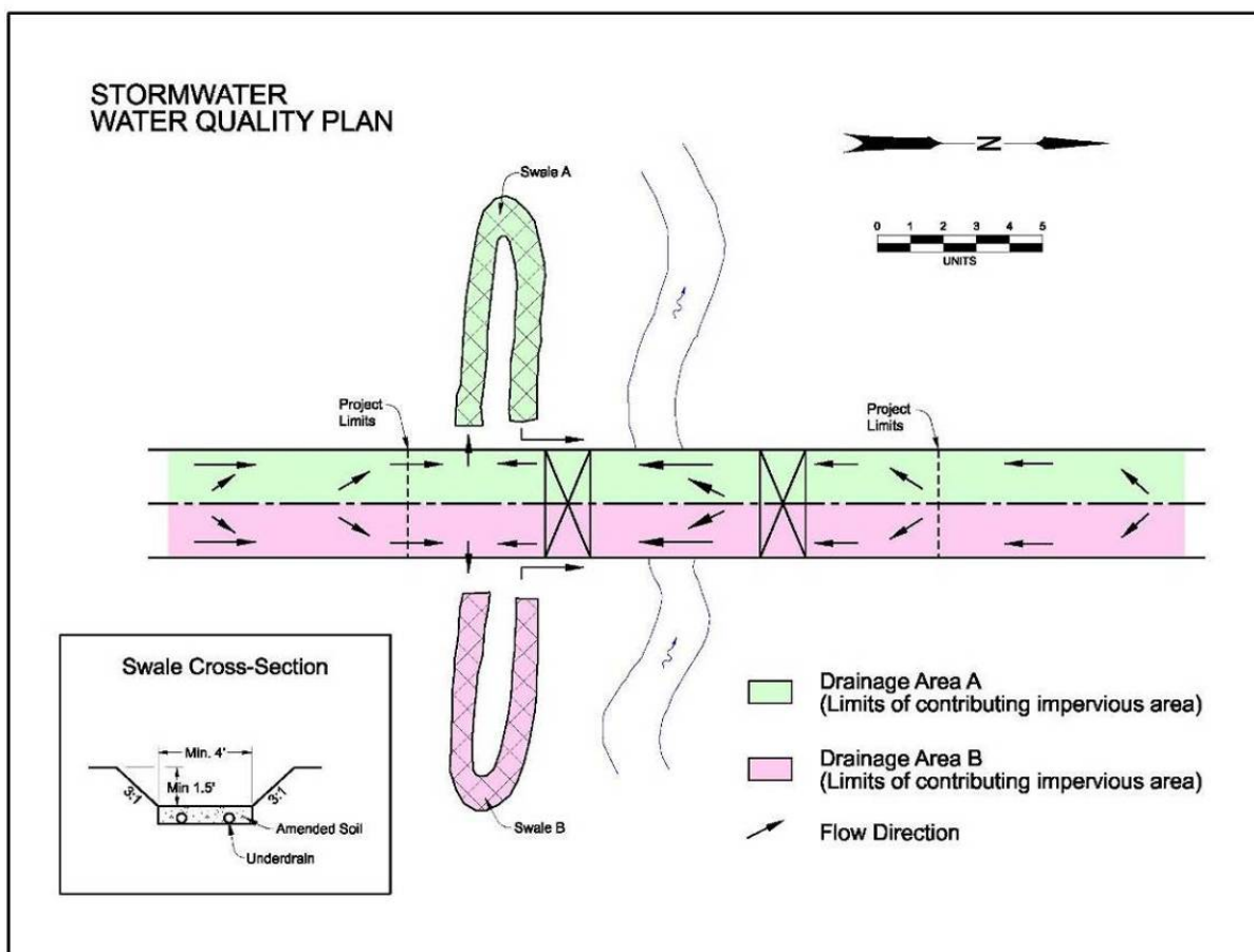
Figure 12. Example stormwater management drawing for a bridge project with water quality treatment provided on the south side of the stream.
