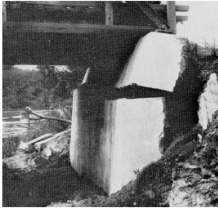
Figure 2.1: Pajaro River Bridge Damage
