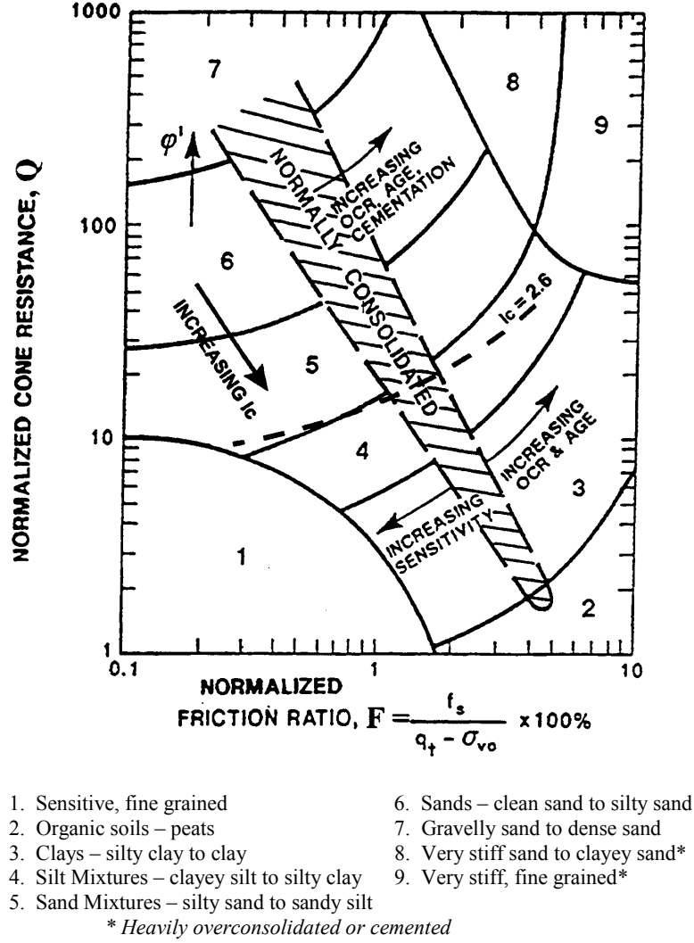
Figure 3.8: Normalized CPT Soil Behavior Type Chart (after Robertson and Wride 1997a, b)
