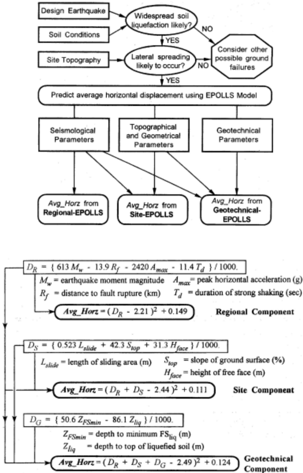
Figure 4.8: Overview of EPOLLS Model for Predicting Average Horizontal Displacement (Avg_Horz) in Meters (Rauch and Martin 2000)
