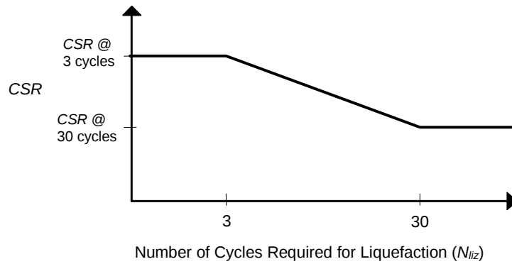
Figure 6.2: Modeled Liquefaction Resistance Curve
