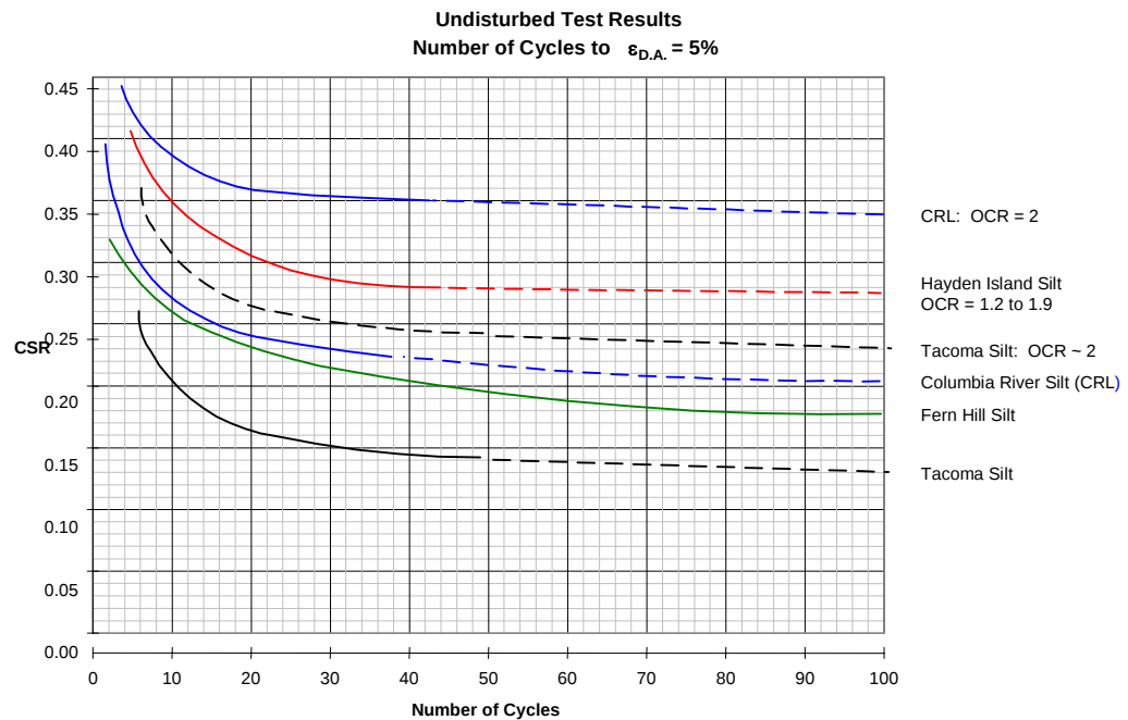
Figure 3.11: Cyclic Resistance Curves for Silty Soils from Various Sites in the Pacific Northwest (after Dickenson and Brown 1997a; Dickenson et al. 2000)
