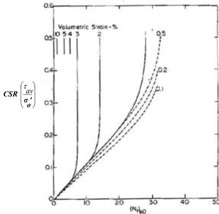
Figure 4.14: Chart for Estimation of Volumetric Strain in Saturated Sands from Cyclic Stress Ratio and Standard Penetration Resistance (Tokimatsu and Seed 1987)
