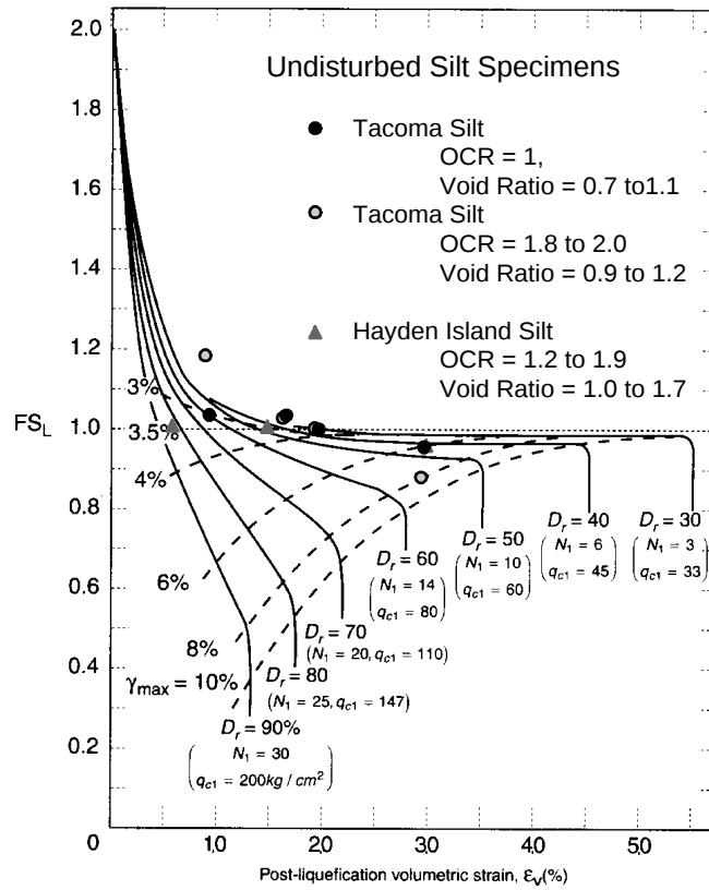
Figure 4.13(a): Factor of Safety versus Volumetric Strain for Undisturbed Silt Specimens
