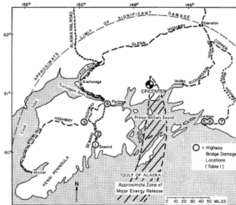
Figure 2.2: Area of Damage of 1964 Alaska Earthquake
