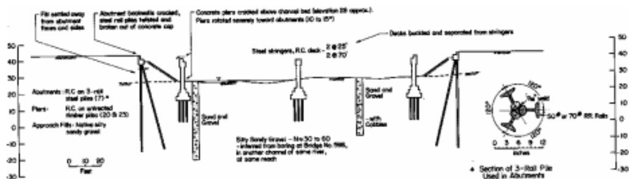
Figure 2.3: Bridge 596, Resurrection River. Centerline Section Looking Upstream (Natural Scale)
