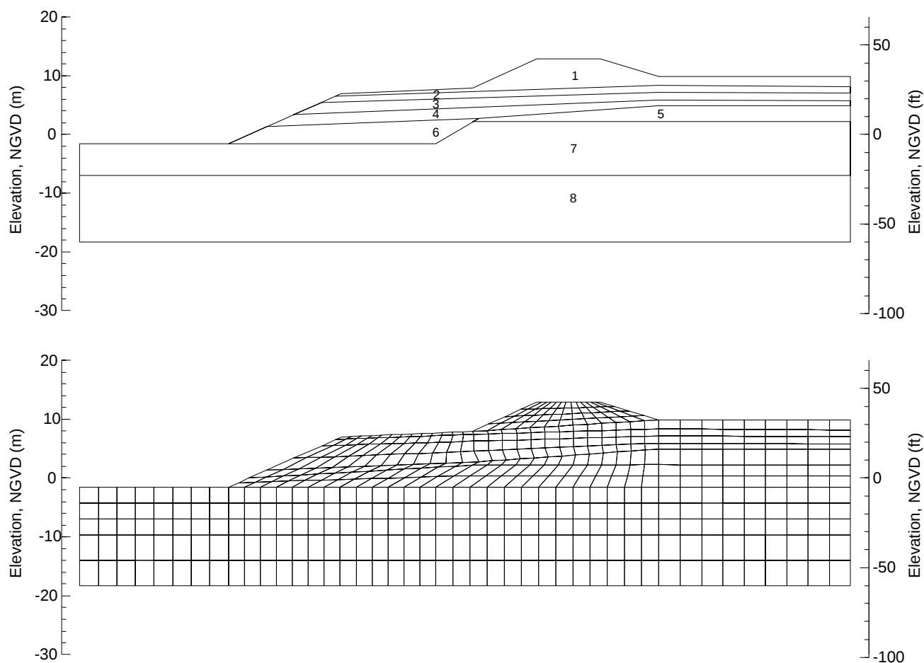
Figure 8.22: The Numerical Model Soil Layering and Grid.
