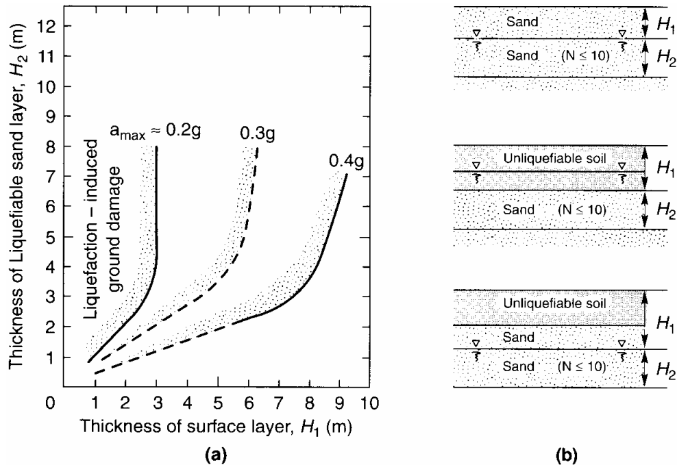
Figure 4.5: (a) Relationship between Thickness of Liquefiable Layer and Thickness of Overlying Layer at Sites for which Surface Manifestation of Liquefaction has been Observed, and (b) Guides to Evaluation of Respective Layer Thicknesses (after Ishihara 1985)
