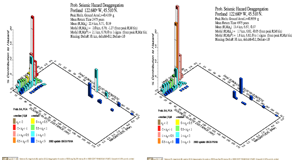
c. 2,475 year mean return time.
