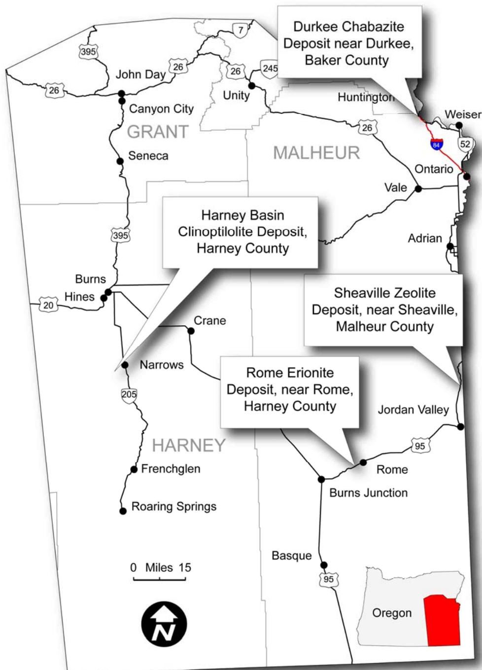
Figure 3.11: Sedimentary zeolites deposits with economic potential in eastern Oregon. The Pliocene Durkee zeolite deposit is about 3 miles east of the Hamlet of Durkee, Baker County. The deposit is an irregular, nearly sinusoidal, 7 mi 2 area of chabazite and subordinate amounts of erionite. To the south in Malheur County, the Sheaville zeolite deposits straddle the Oregon-Idaho border and composed of clinoptilolite- and chabazite-bearing silicic tuffs. The zeolite deposits just west of Rome, Malheur County, have replaced the Miocene Rome beds over an elongated north-south 220 mi 2 area. Some of these beds consist entirely of erionite; but other beds are mordenite- or phillipsite-bearing. A high-grade clinoptilolite deposit called the Harney Basin deposit is just west of the Narrows (Harney County); both phillipsite and erionite occur locally with clinoptilolite
