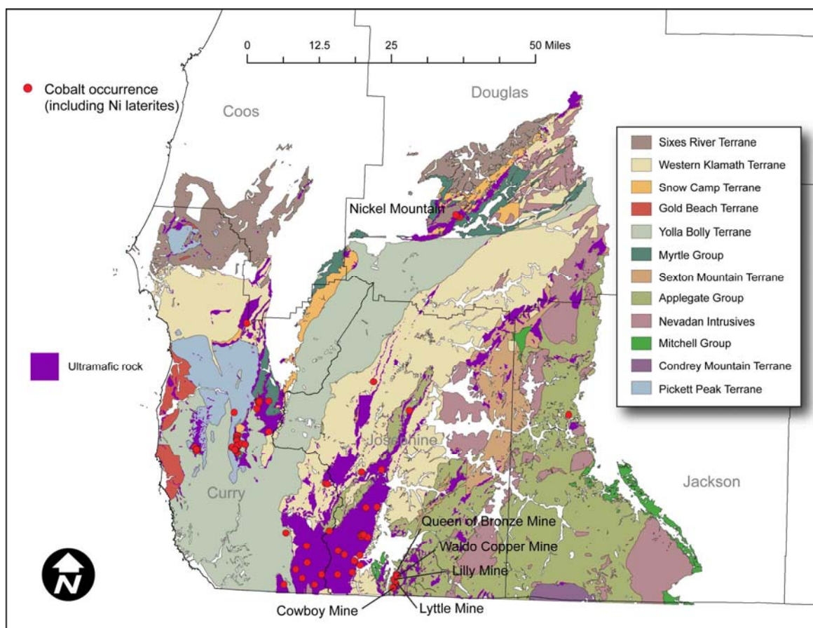
Figure 3.6: Cobalt-bearing deposits in southwestern Oregon
