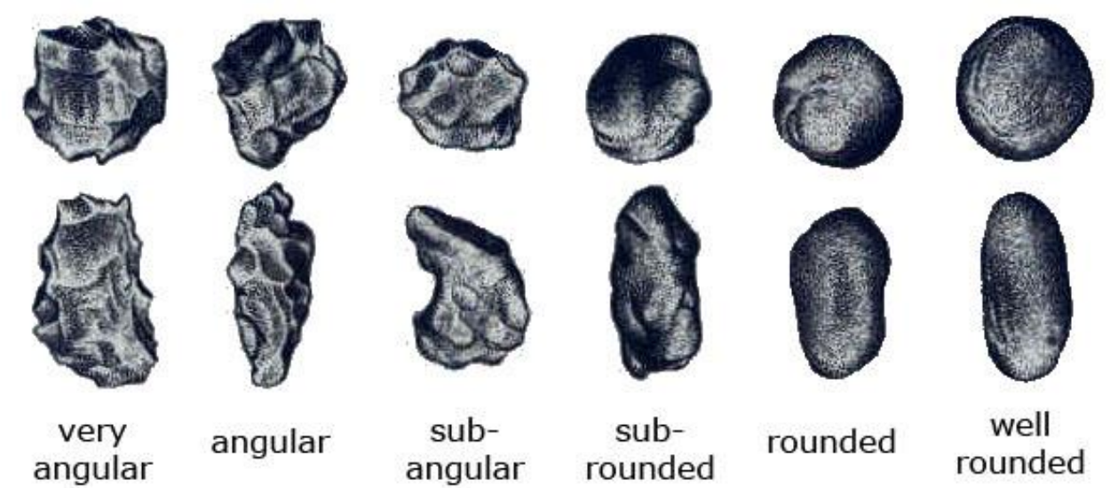
Figure 5-4 Particle Shape for Coarse-Grained Soil Particles
