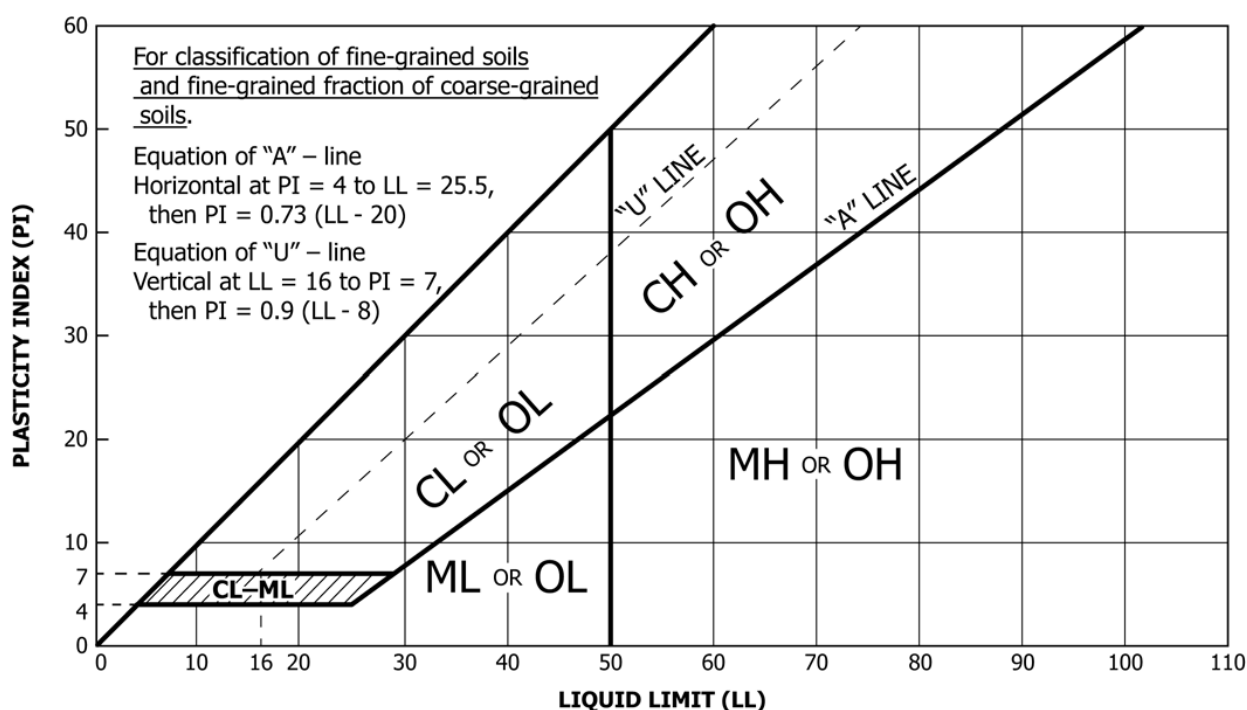
Figure 5-1 Plasticity Chart
