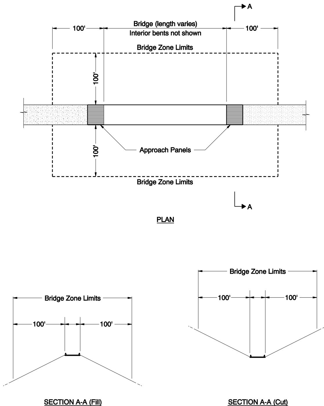
Figure 16-1 Bridge Zone
