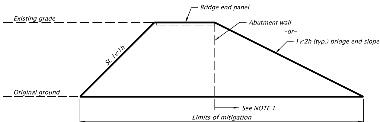
Figure 13-15 Extent of Ground Improvement for Liquefaction Mitigation
