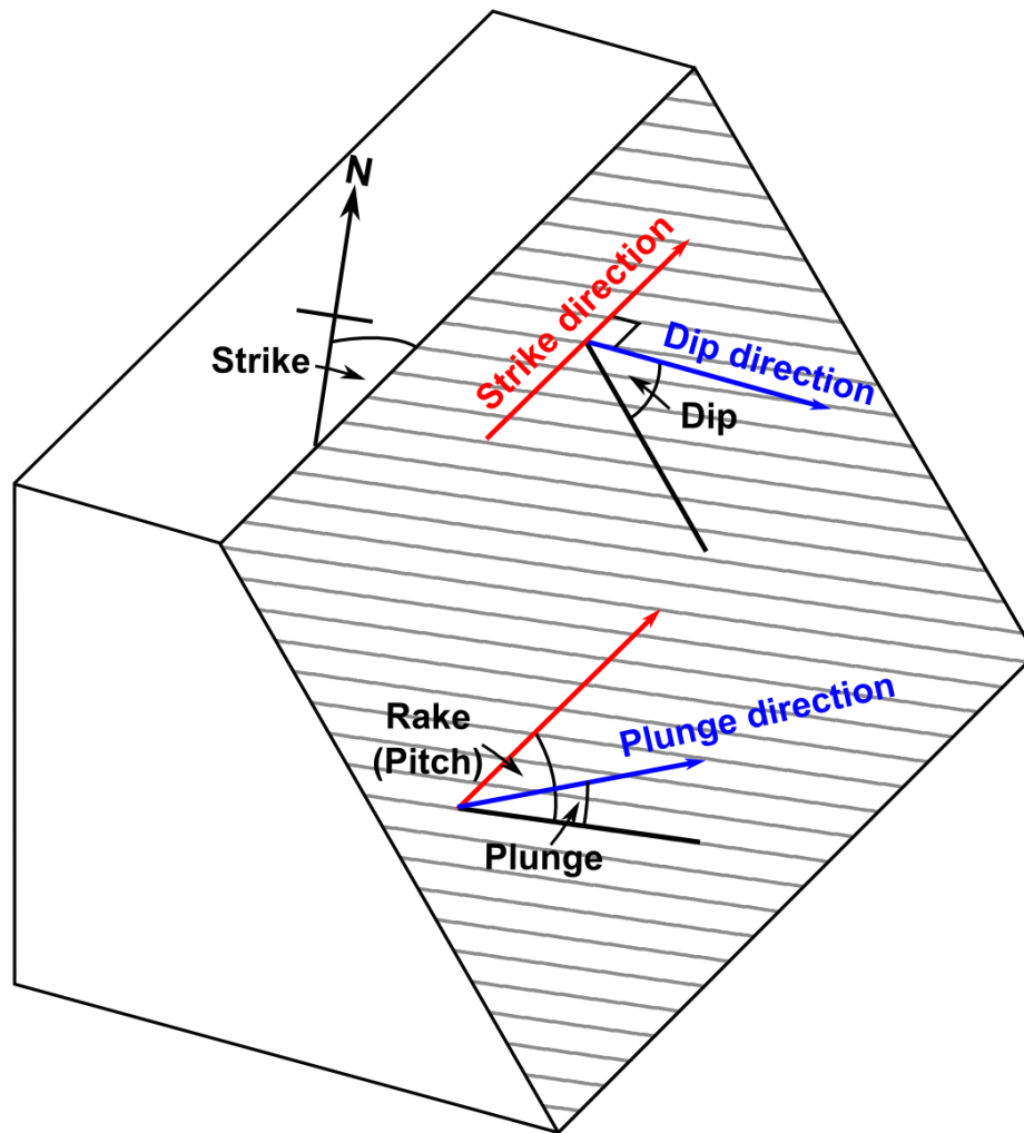
Figure 5-6 Orientation Measurements of Planar and Linear Features
