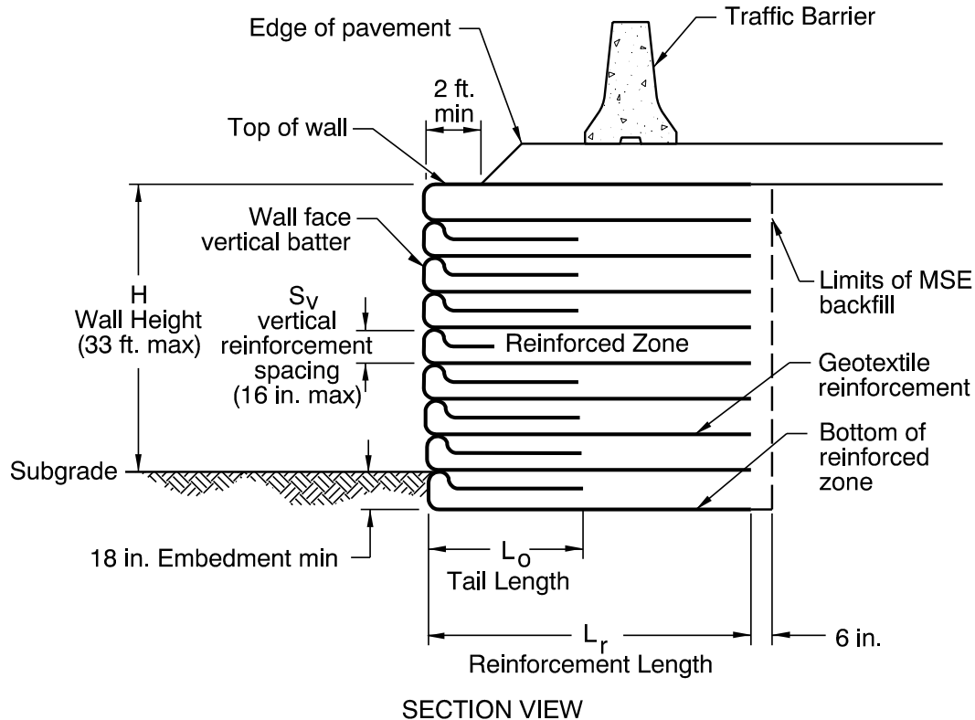
Figure 16-7 Temporary Geotextile-Reinforced MSE Wall
