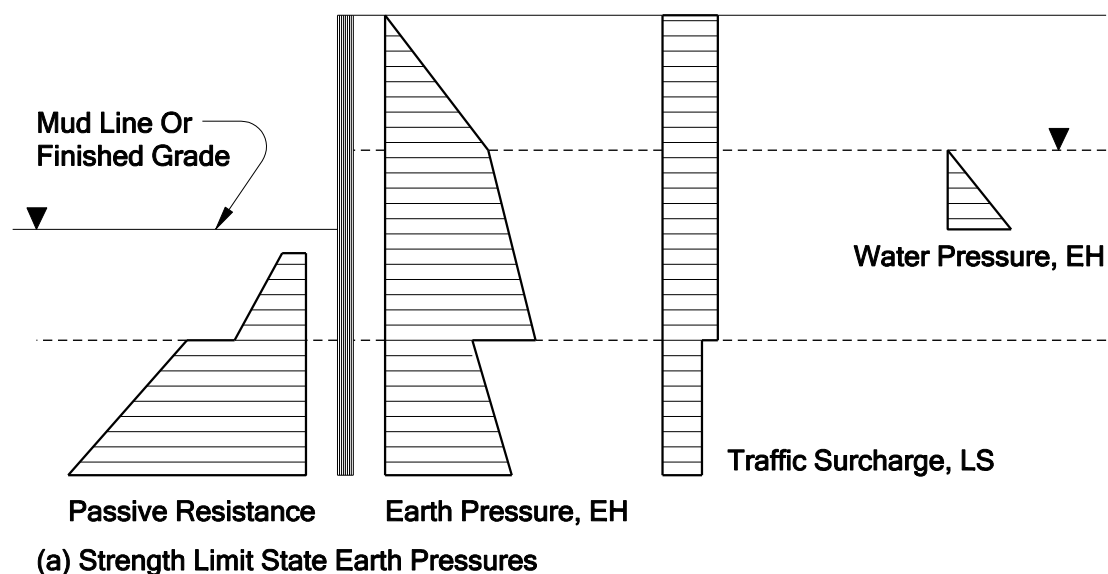
Figure 20-6 Example presentation of lateral earth pressures for non-gravity cantilever and anchored wall design.
