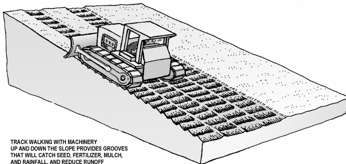
Figure 3-17 Surface Roughening
