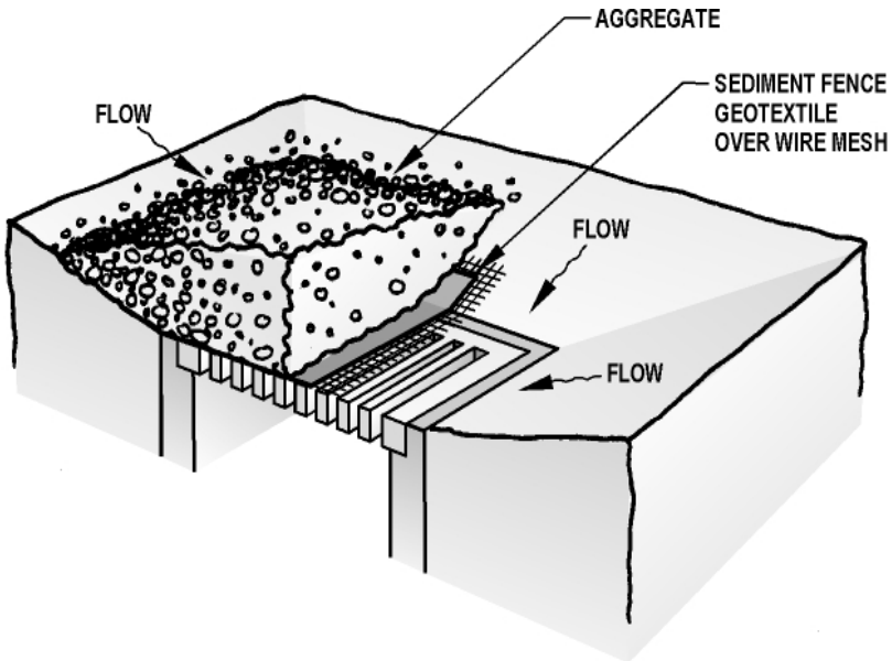
Inlet Protection - Geotextile/Wire Mesh/Aggregate (Type 2)
