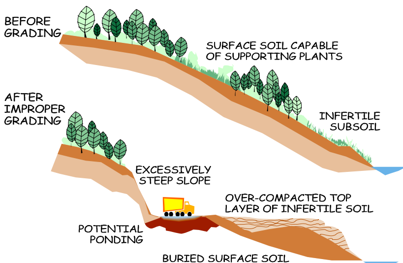
Figure 2-1 Fit construction to the natural contours of the land
