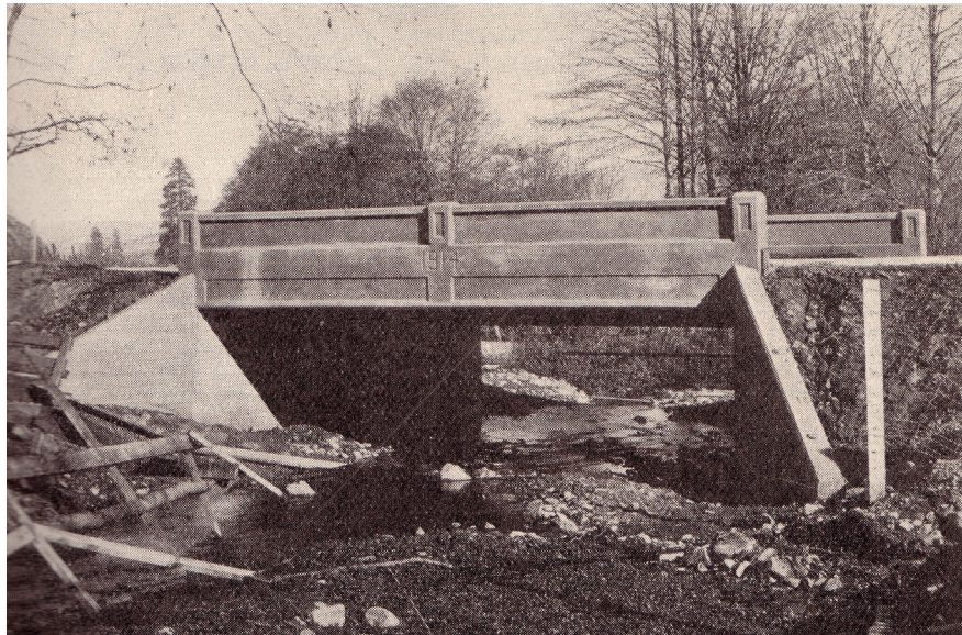
Figure 1.9. “Type of Concrete Bridge Erected Along Pacific Highway in Jackson County”
