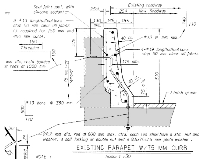
Figure 2.15. Type F Retrofit of Existing Bridge Rail (shown in shade clarity) Source: ODOT Drawing, BR283
