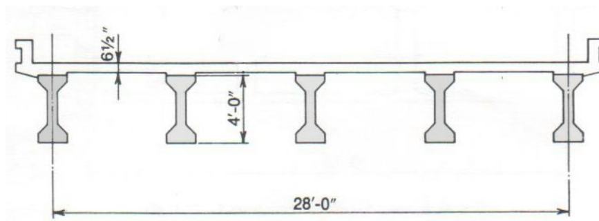
Figure 1.18. Typical Pre-cast “T” Girder/Beam Bridge Section Source: Libby & Perkins (1976)
