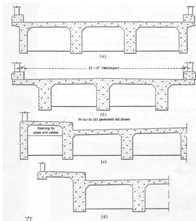
Figure 1.16. Typical Concrete Deck Girder Sections
