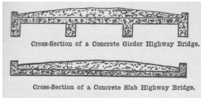
Figure 1.15. Girder and Slab bridges in Section
