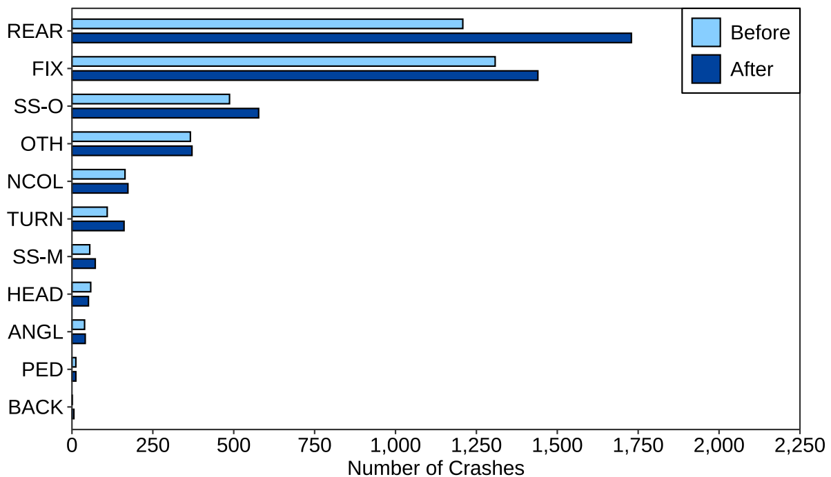
Figure 3.13: Number of Crashes by Crash Type on Control and Speed Reduction Segments
