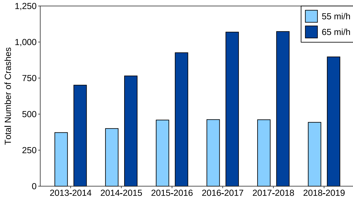
Figure 3.5: Total Crashes by Year and Speed Limit Group at Control Locations
