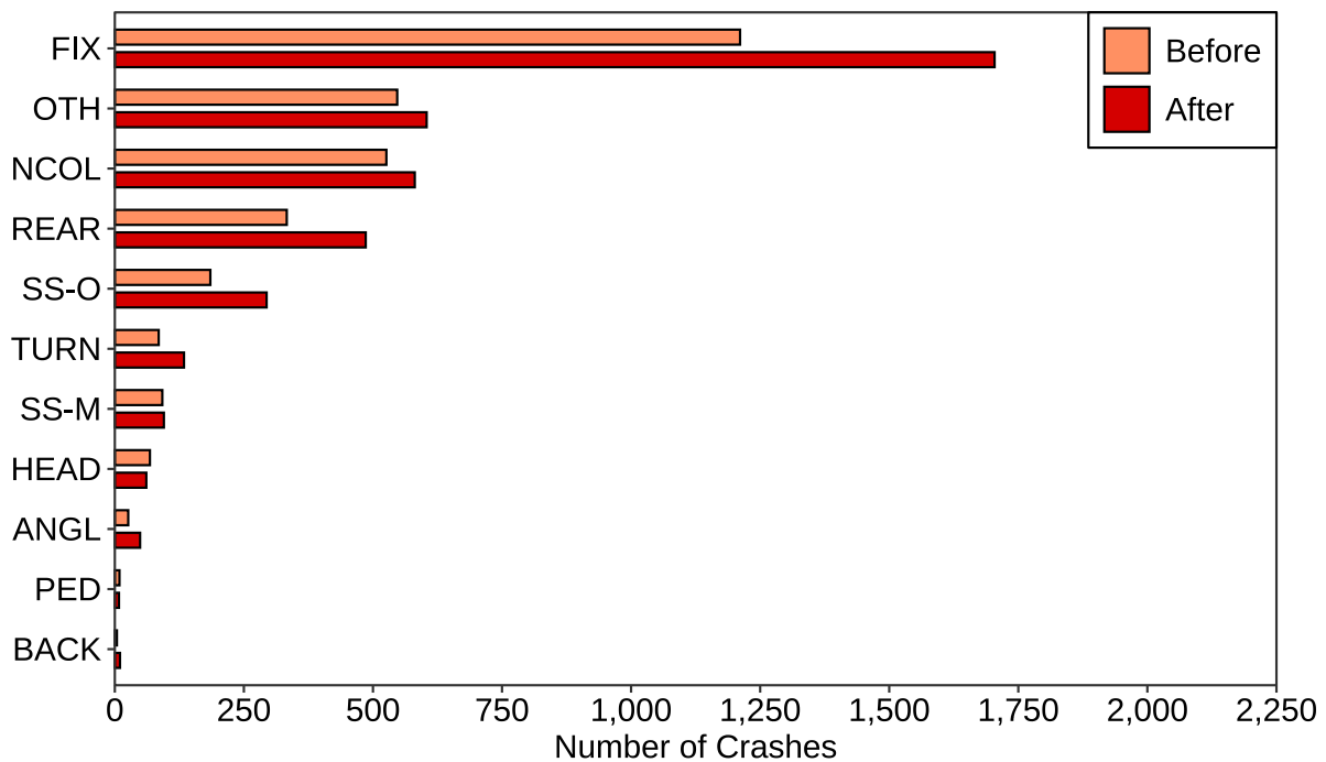
Figure 3.14: Number of Crashes by Crash Type on Increased Speed Limit Segments
