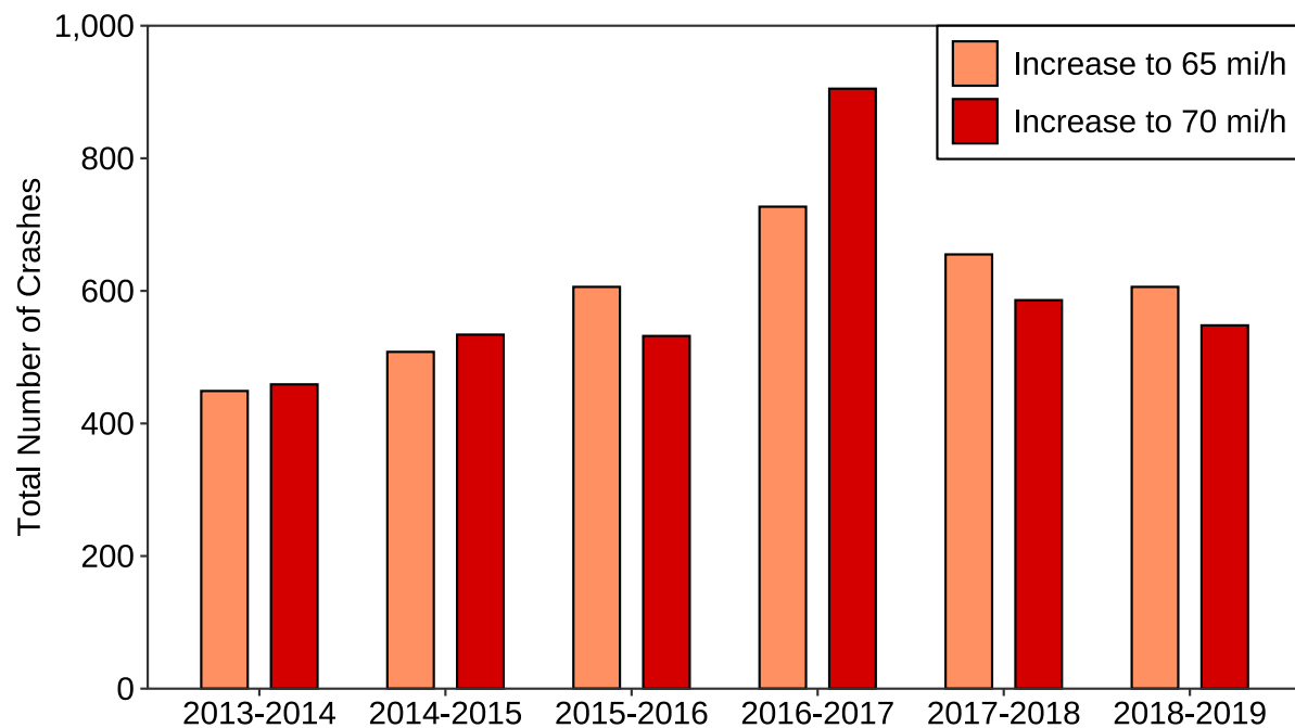
Figure 3.6: Total Crashes by Year and Speed Limit Group at Increased Speed Limit Locations
