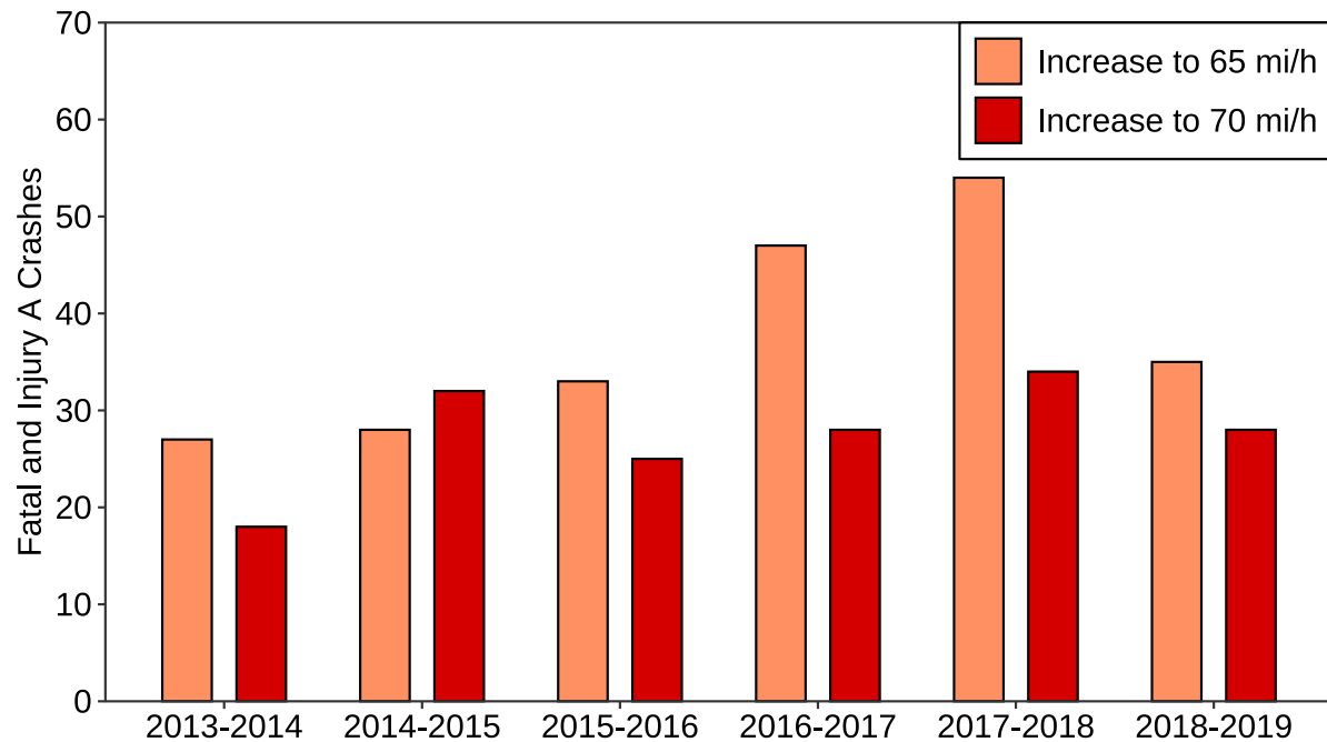
Figure 3.8: Fatal and Injury A Crashes by Year and Speed Limit Group at Increased Speed Limit Locations
