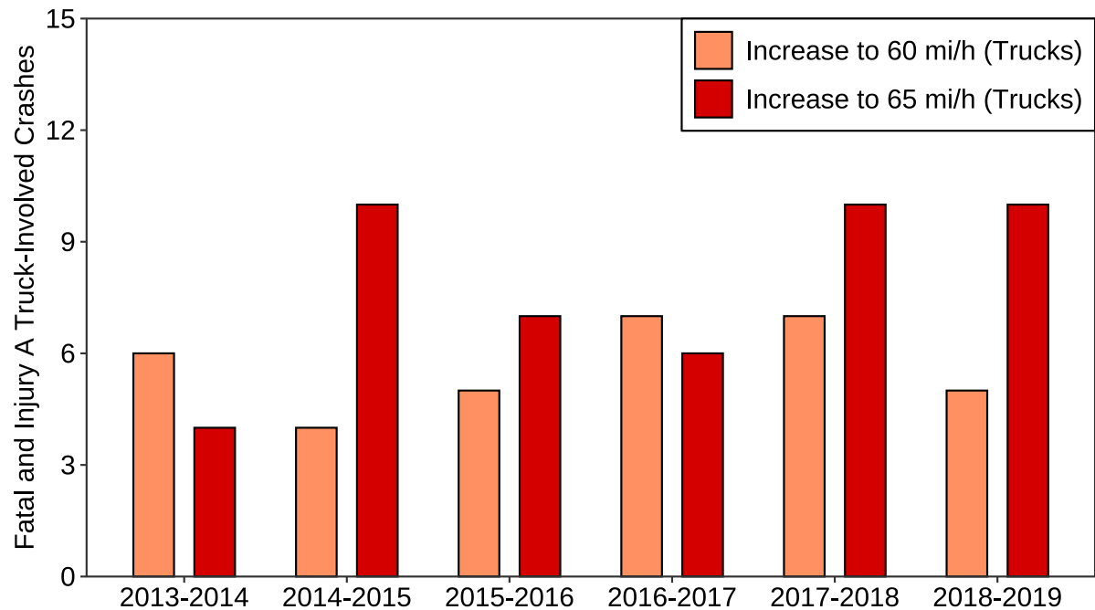
Figure 3.12: Fatal and Injury A Truck-Involved Crashes by Year and Speed Limit Group on Increased Speed Limit Segments
