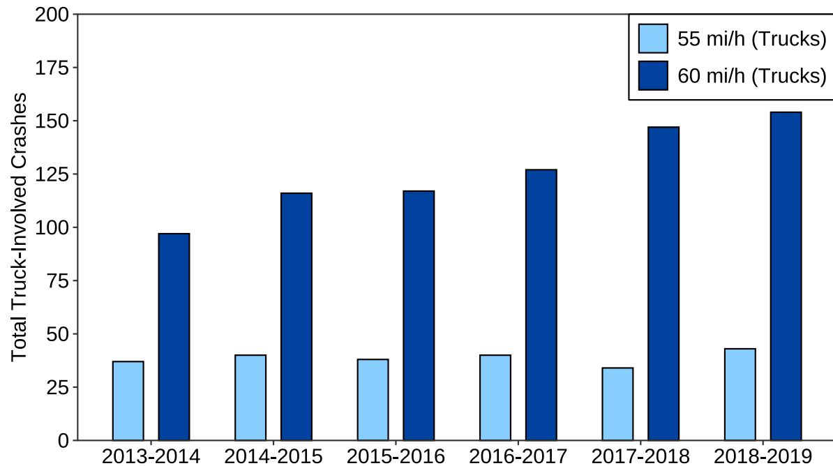
Figure 3.9: Total Truck-Involved Crashes by Year and Speed Limit Group on Control Segments
