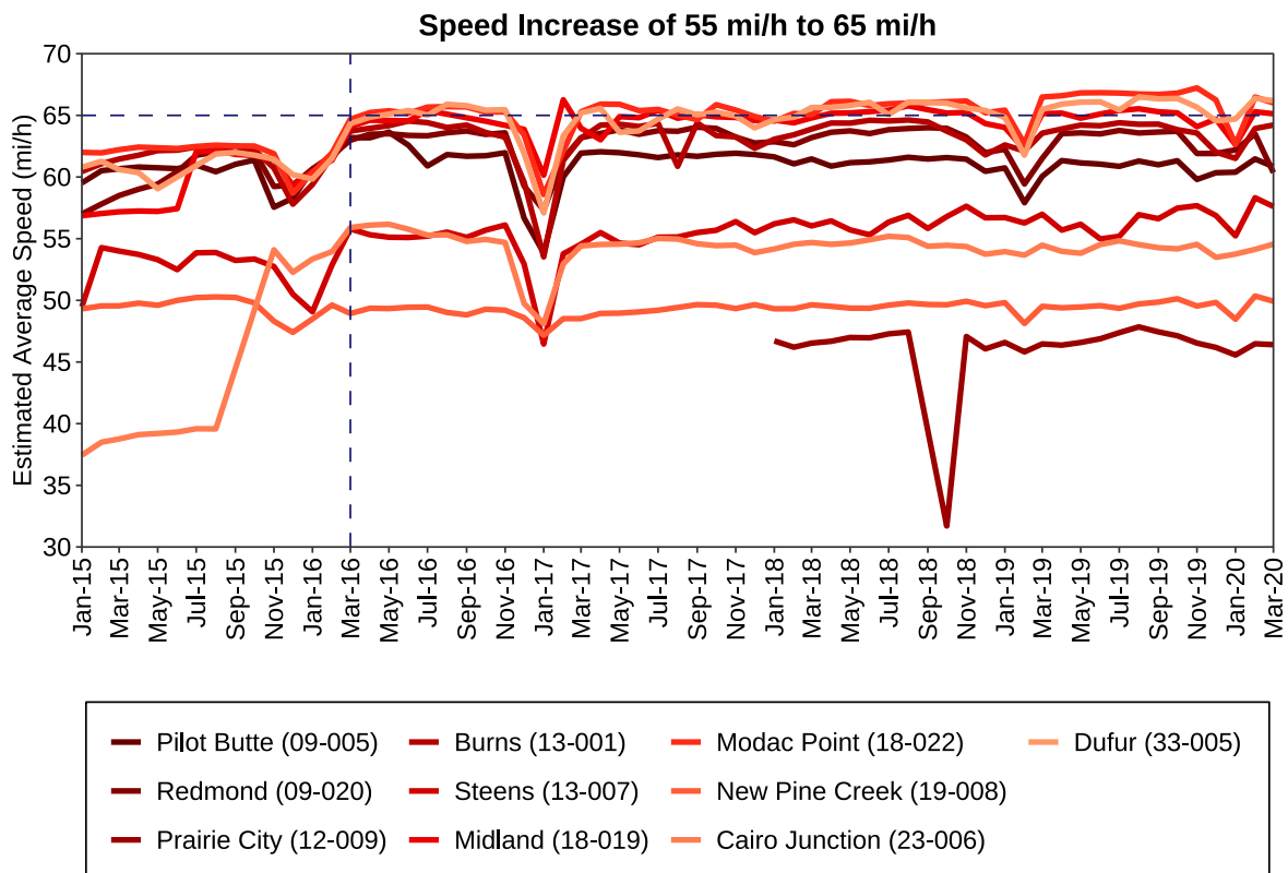
Figure 3.2: Average Monthly Speed Plots for Increased Speed Limit Segments
