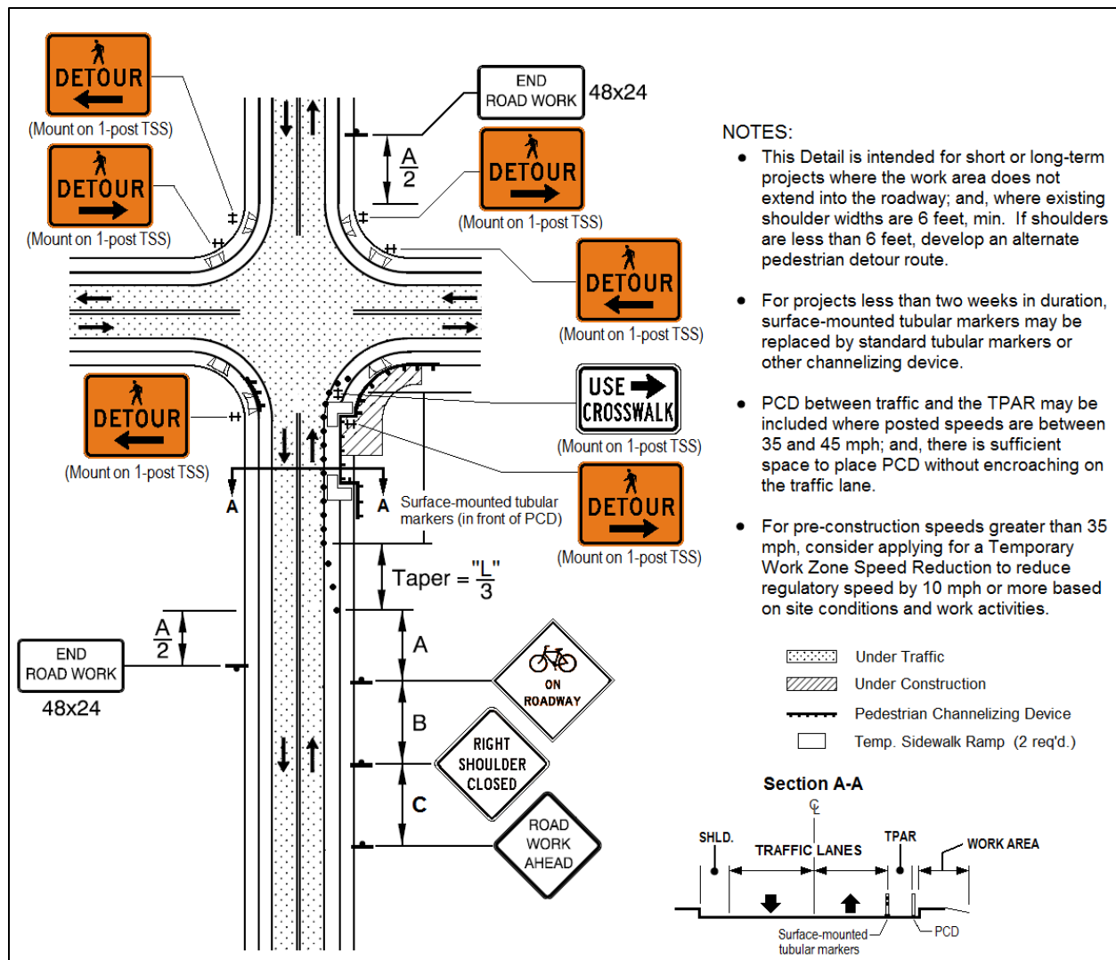
Figure A-10: TPAR On-Site Diversion onto Shoulder or Bicycle Lane
