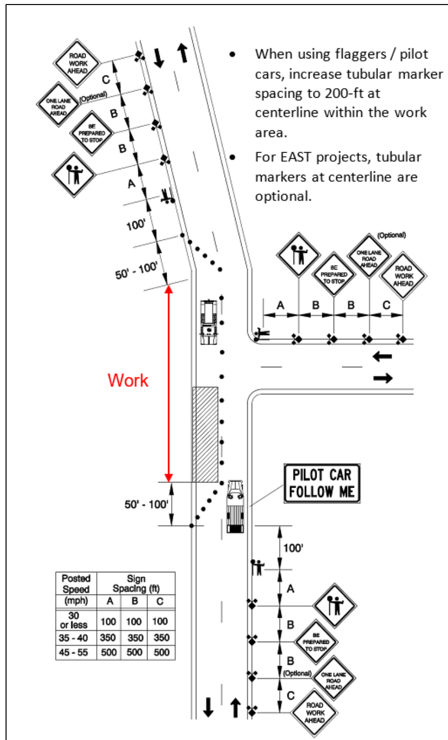
Figure A-2: Flagging Operation with Pilot Car
