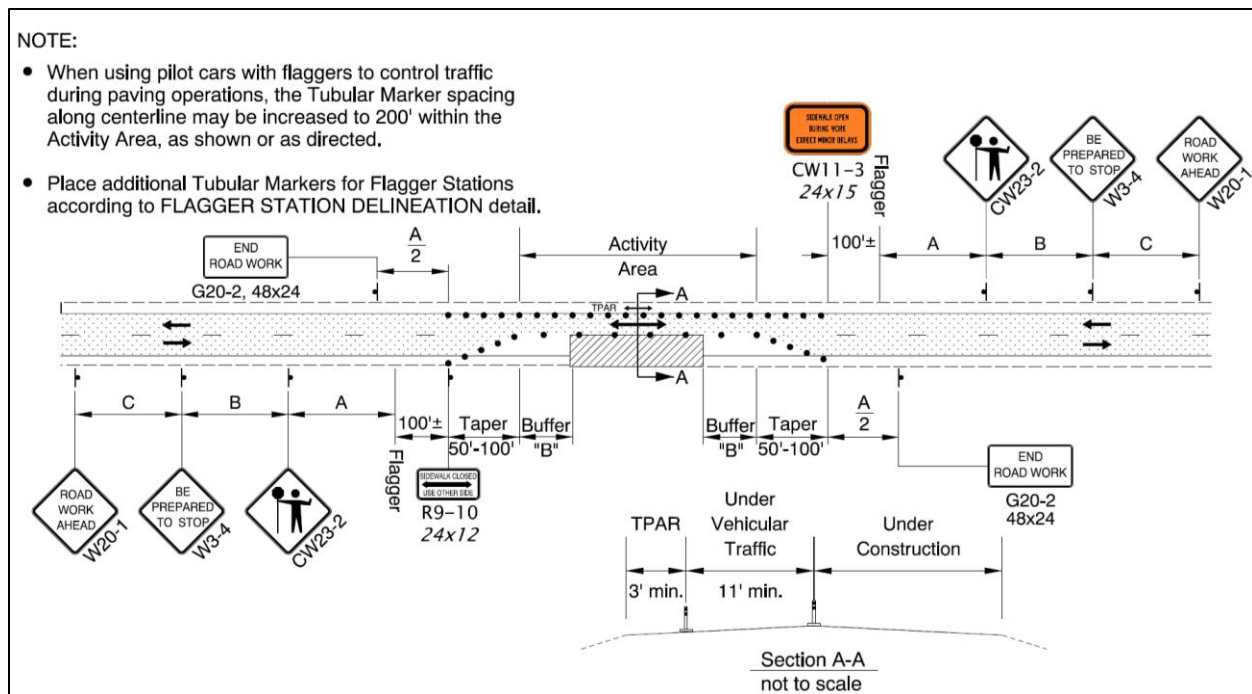
Figure A-12: TPAR – 2-Lane, 2-Way Roadway – One Lane Closure
