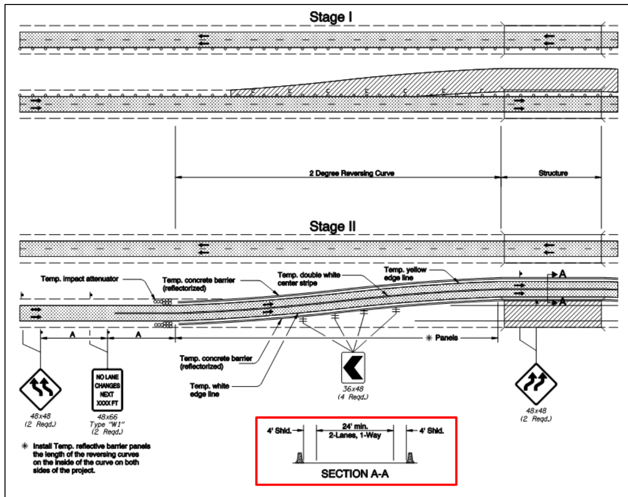
Figure A-2: TCP Staging of On-Site Diversion
