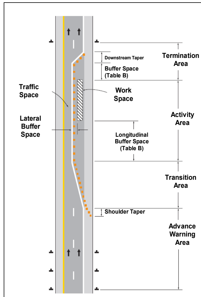
Figure A-1: Work Zone Components
