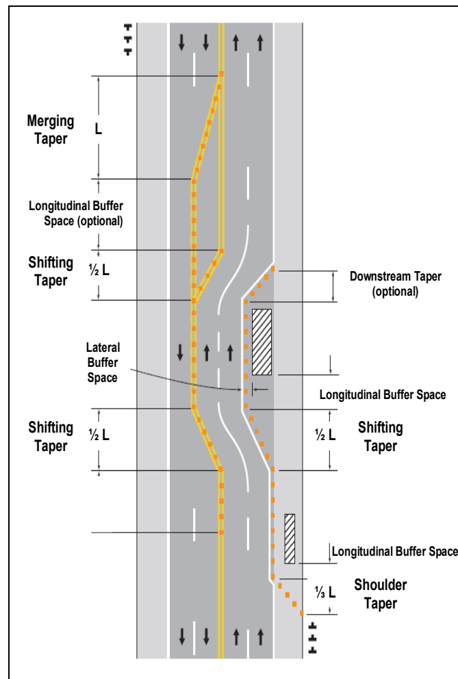
Figure A-2: On-Site Diversion
