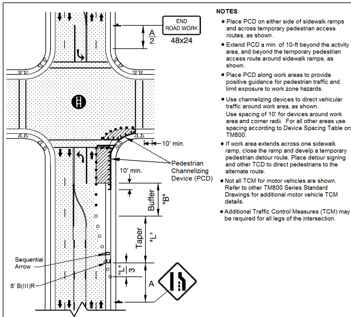
Figure A-9: TPAC at Existing Signalized, Marked Crosswalk
