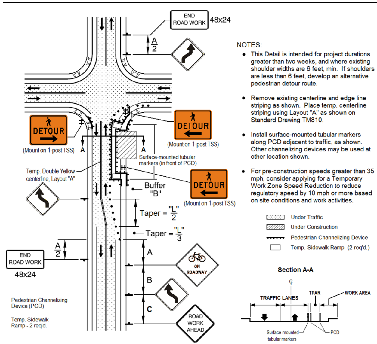
Figure A-11: TPAR – On-Site Diversion with Partial Traffic Lane Encroachment
