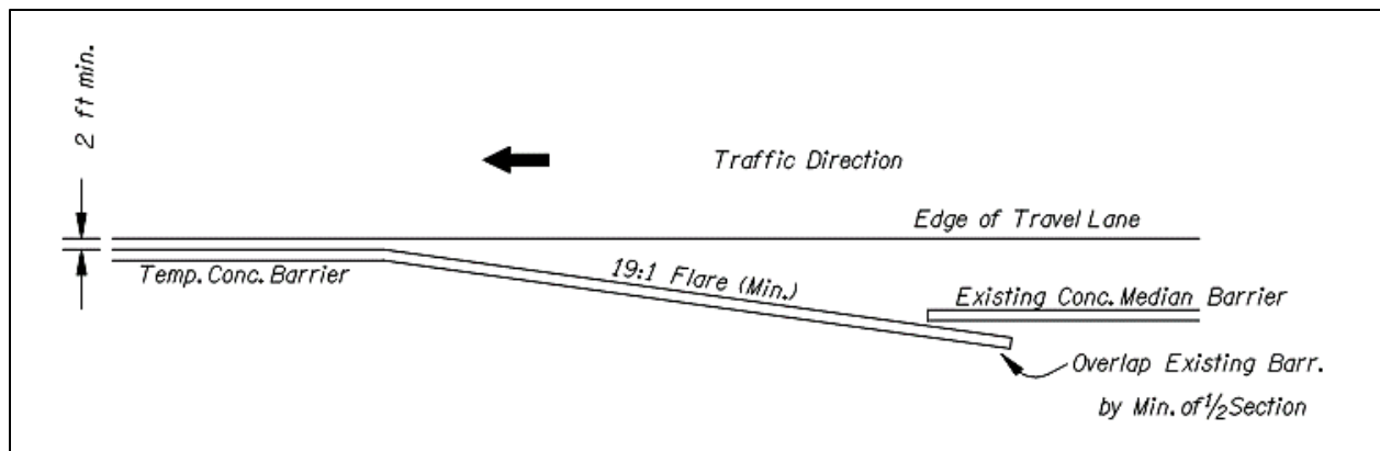
Figure A-2: Typical Overlap of Temporary Concrete Barrier
