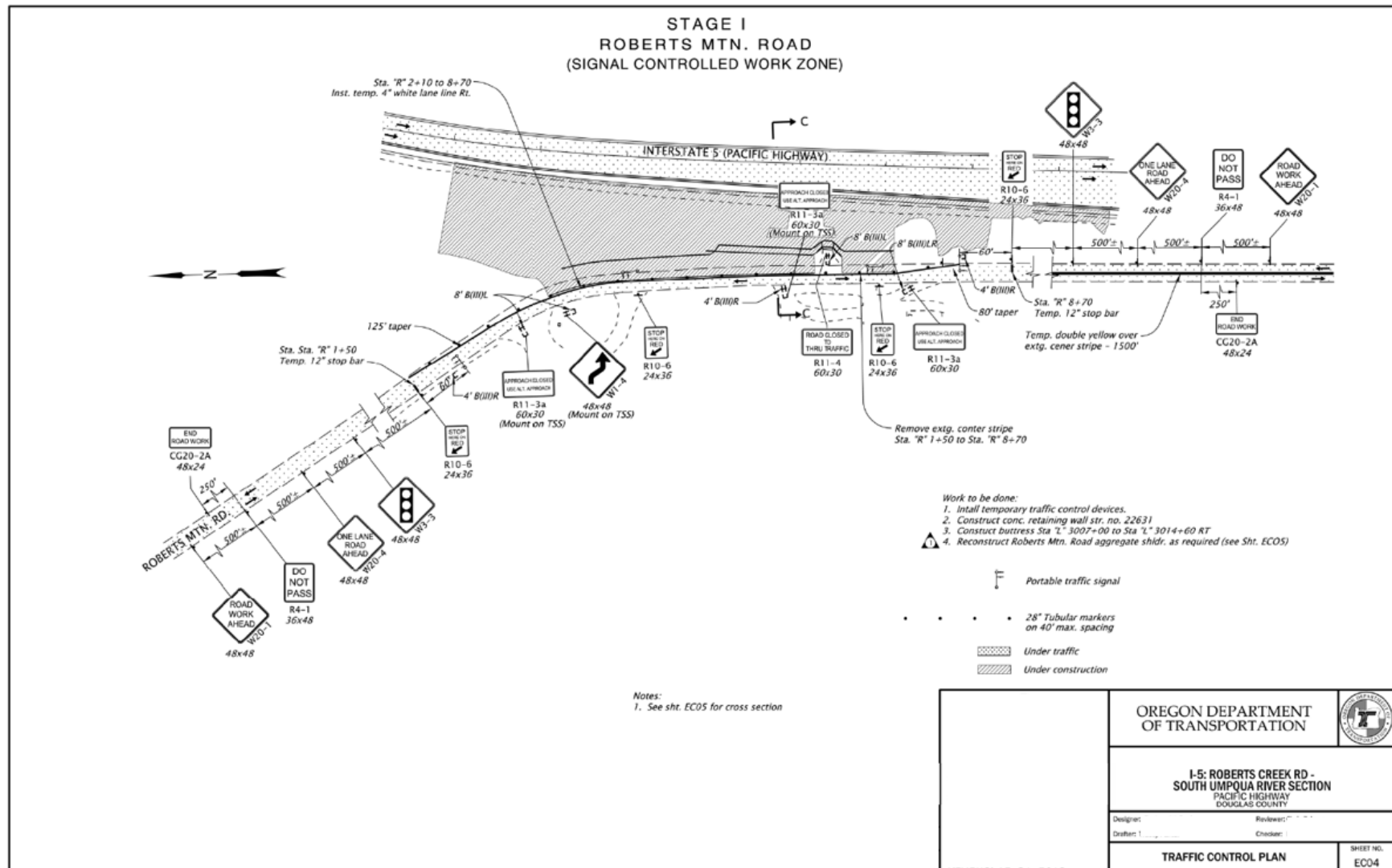
Figure A-4: Staging Plan Sheet
