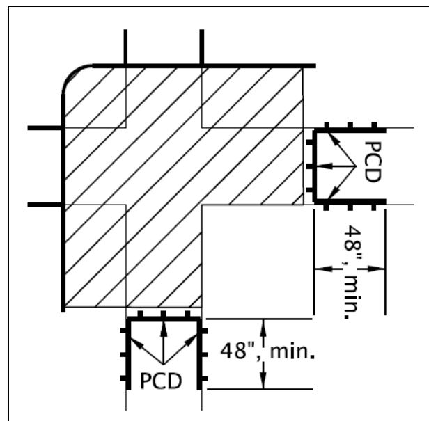
Figure A-3: PCD Closure Detail
