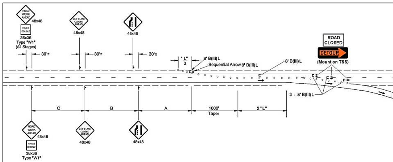
Figure A-2: Freeway Closure
