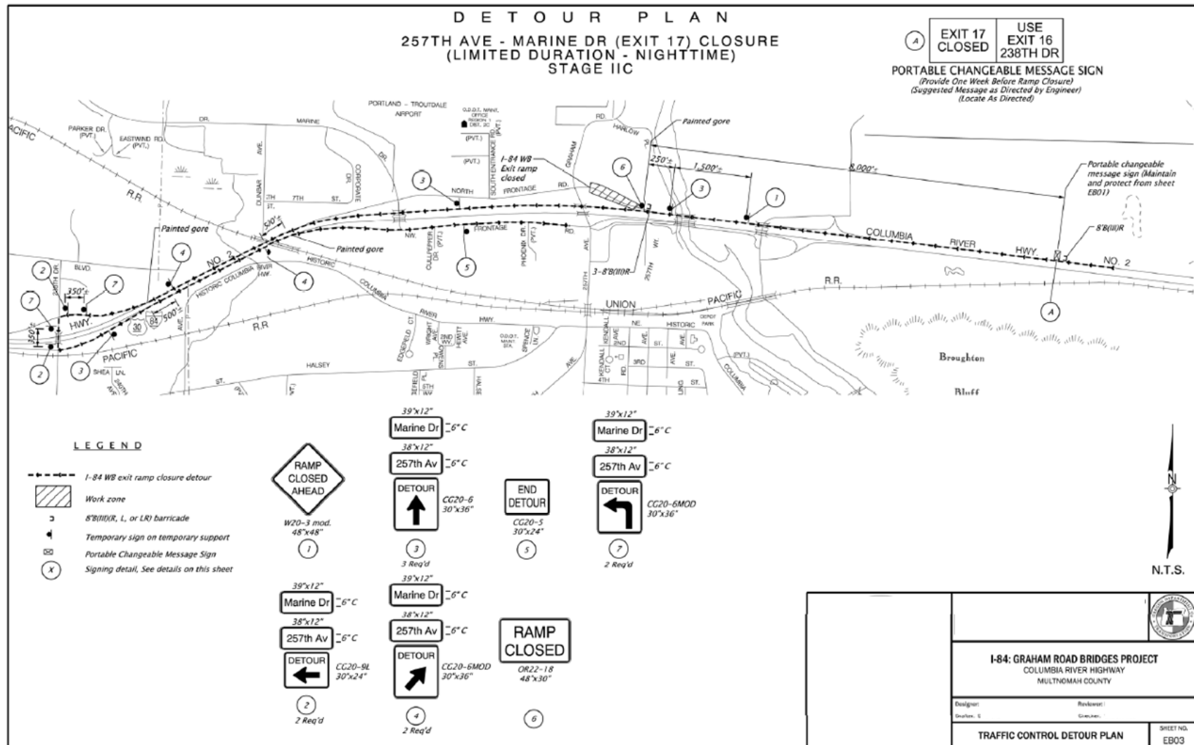
Figure A-2: Detour Sheet
