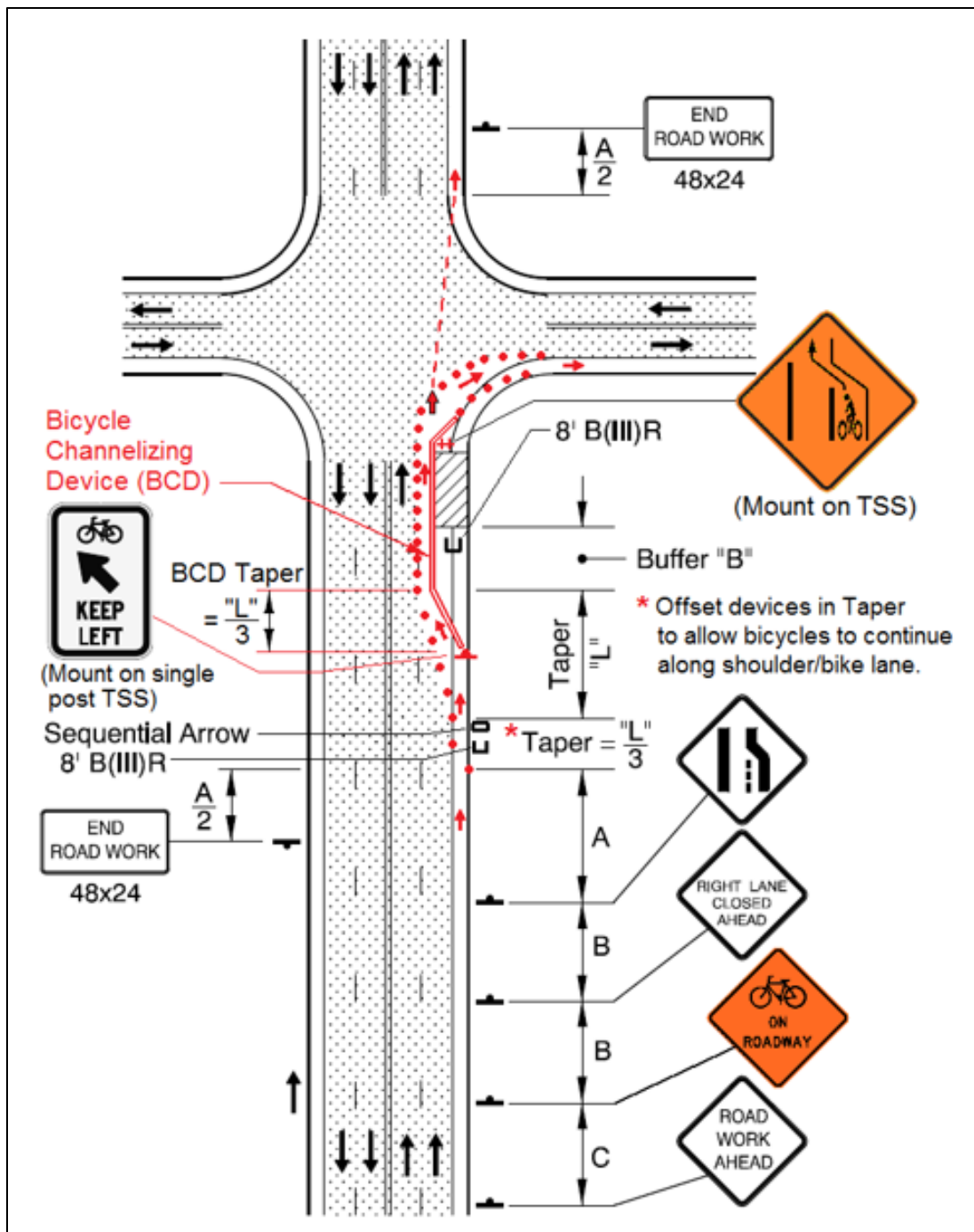
Figure A-5: Suggested BCD Usage
