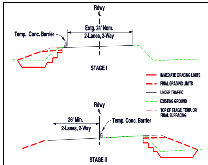
Figure A-2: Cross Section Example
