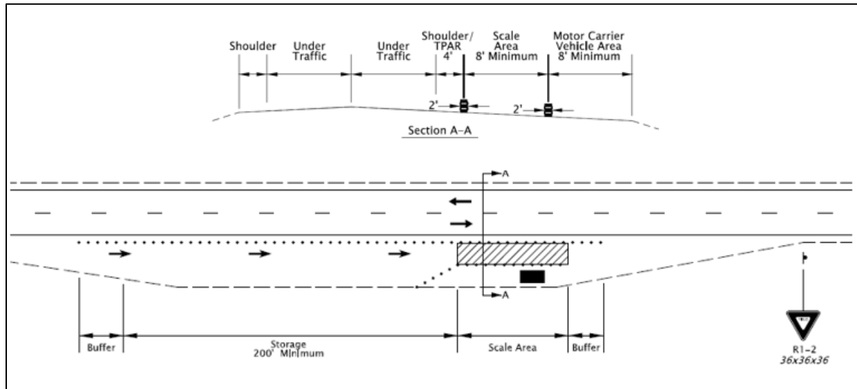
Figure A-2: Temporary Weigh Stations and Chain up Areas Layout
