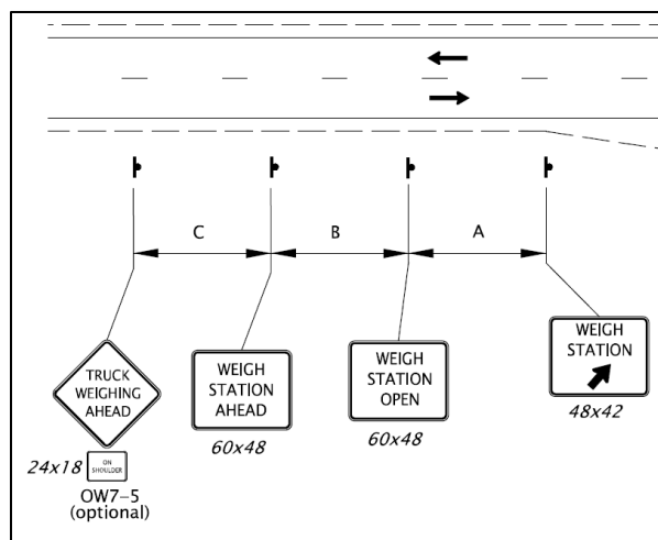
Figure A-1: Advance Signing for Enforcement Areas
