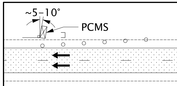
Figure 9 - Rotate the PCMS to improve legibility
