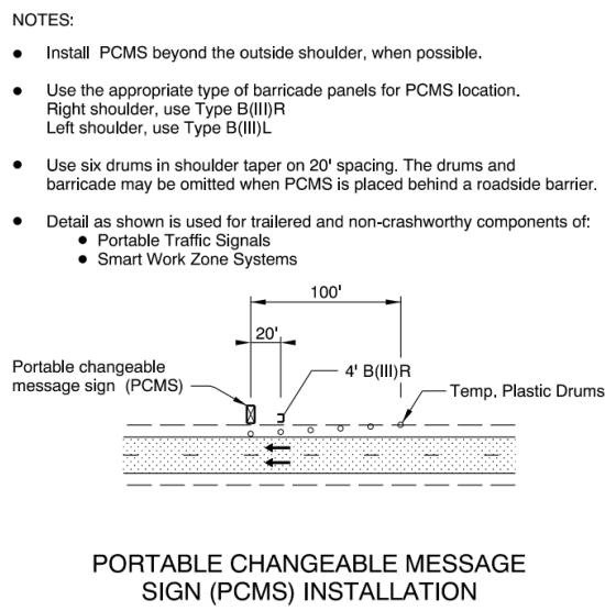
Figure 4 - TM800 PCMS installation detail.
