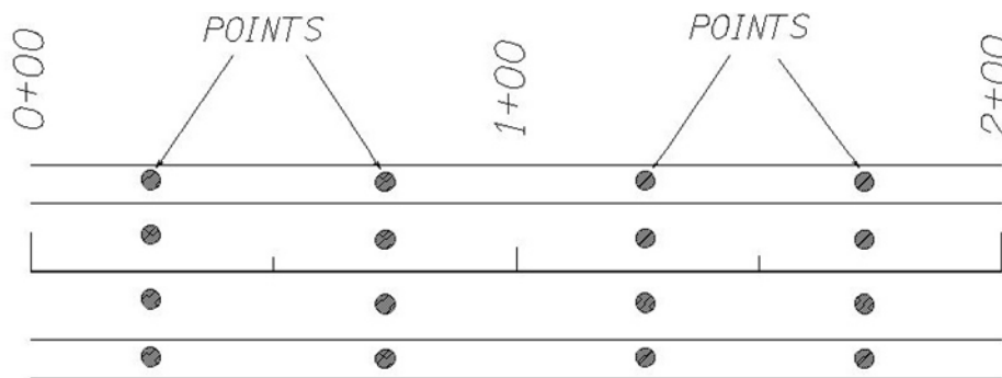
Figure 1: Sample Grade Verification Point Layout using Cross Section Method on a +/- 40-foot-wide Section
