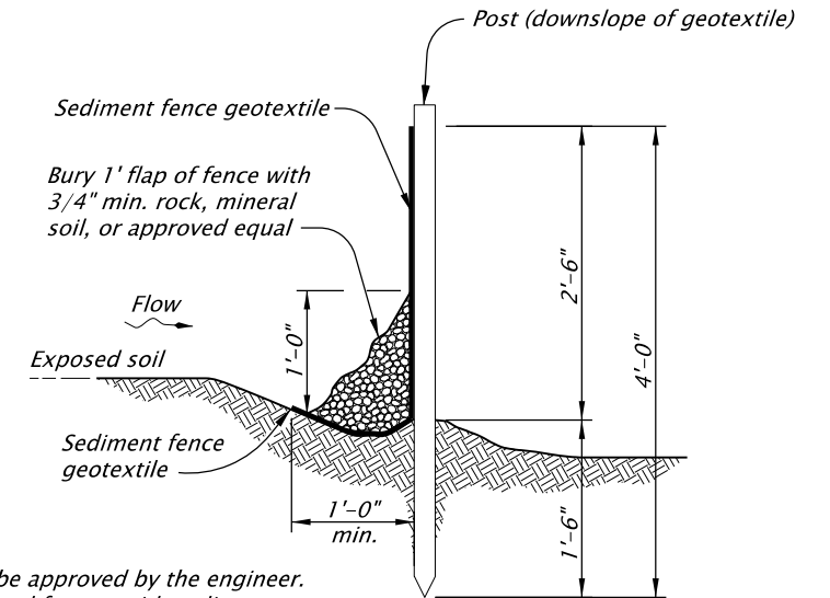
ALTERNATE SEDIMENT FENCE WITHOUT TRENCHING - TYPE 2 NOT TO SCALE
