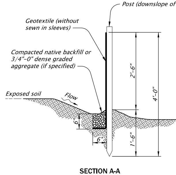
SEDIMENT FENCE AND GEOTEXTILE BURY DETAIL - TYPE 1 NOT TO SCALE
