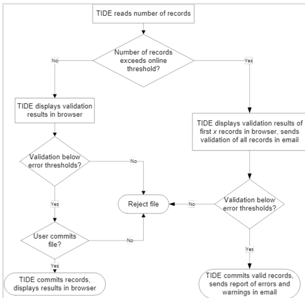
Figure 86. Upload Processing Flow
