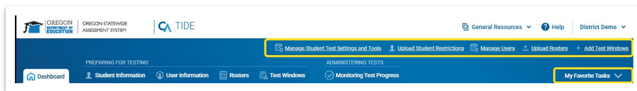
Figure 19. Favorite Tasks
