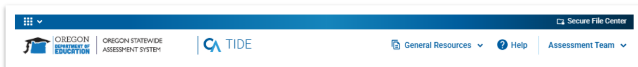
Figure 18. Header
