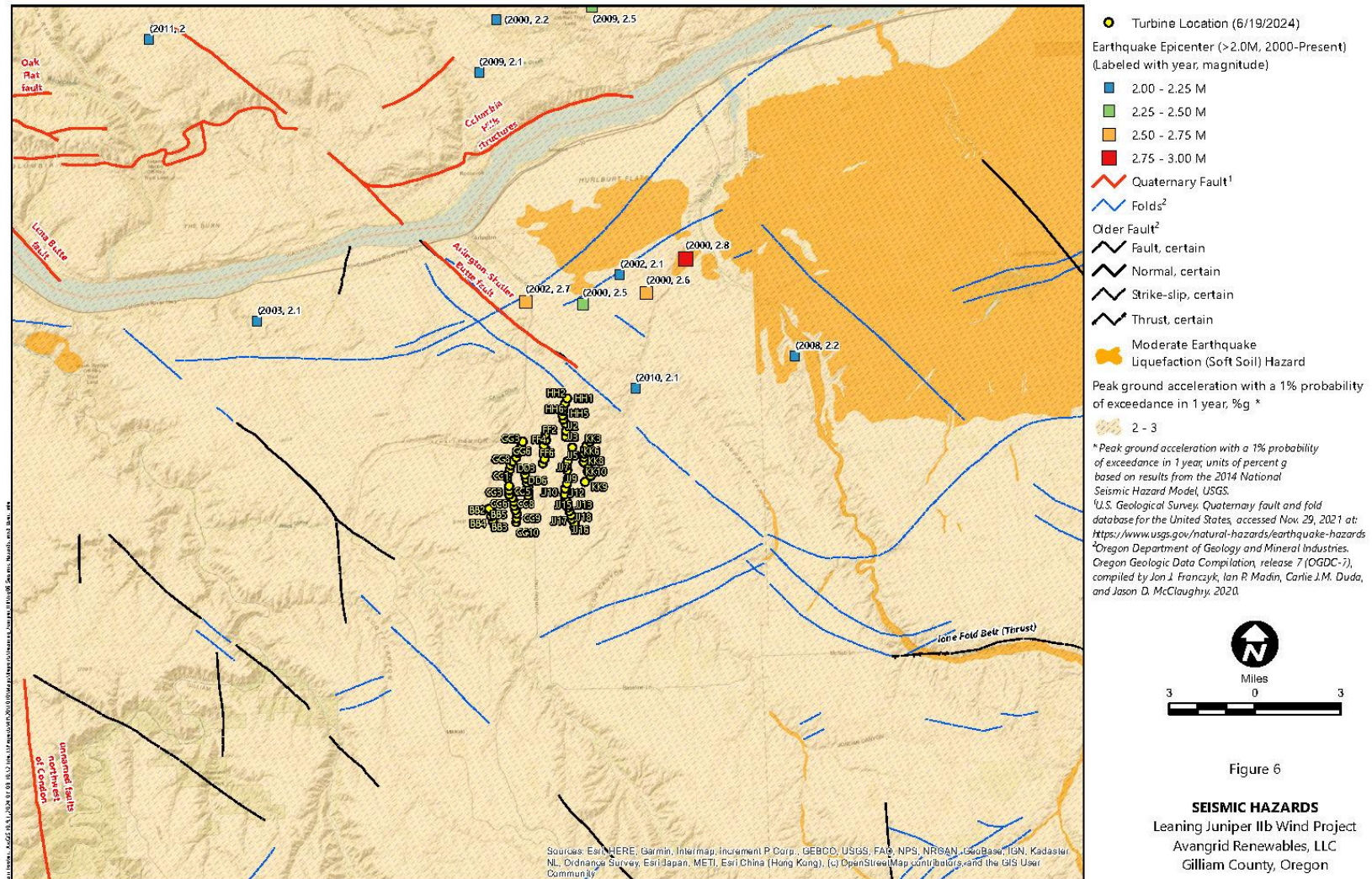
Figure 3: Seismic Hazards within the Analysis Area
