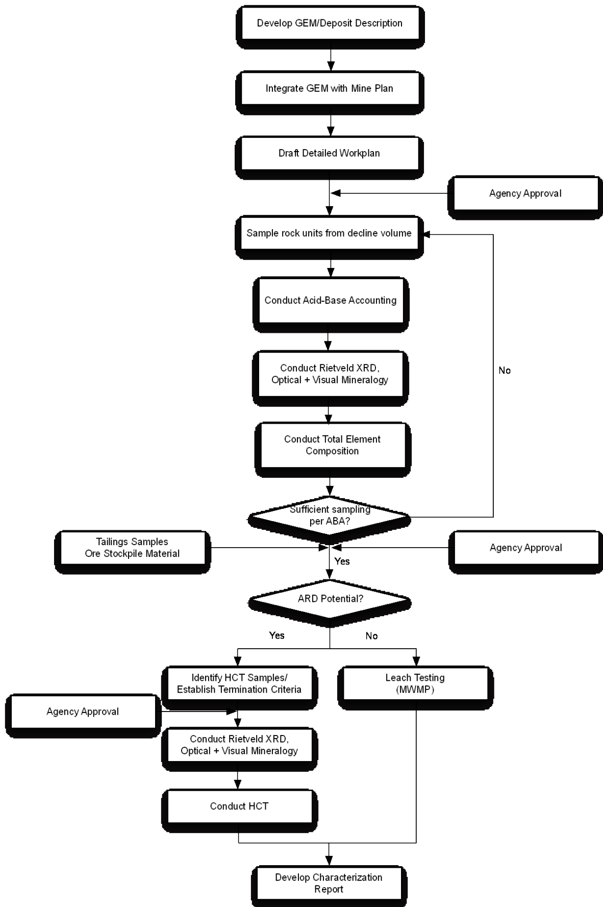
Figure 7 Workflow for Geochemical Characterization Plan
