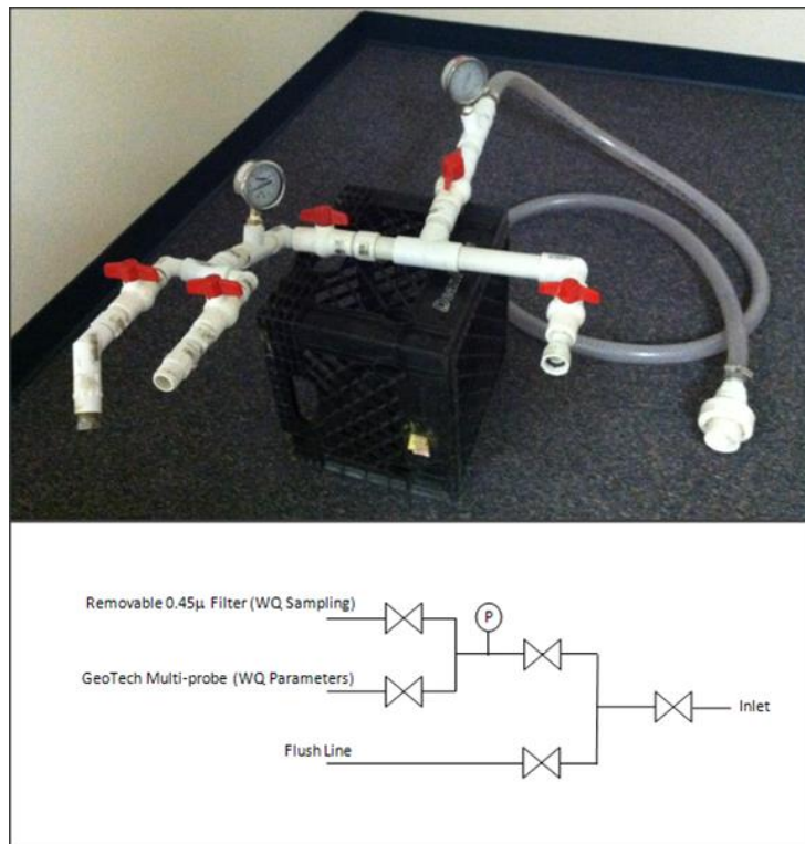
Photo 1. Discharge testing manifold photograph and diagram
