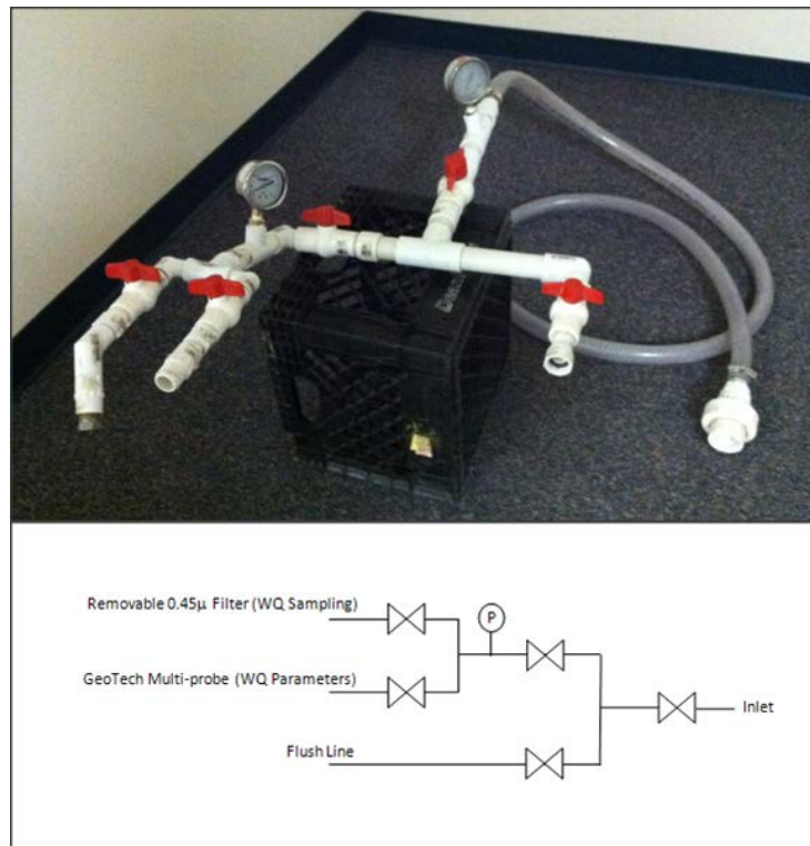
Figure 1. Discharge testing manifold photograph and diagram
