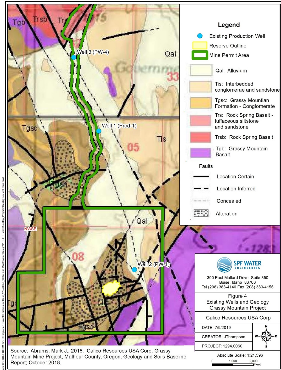
Figure 4. Map of existing wells and surficial geology
