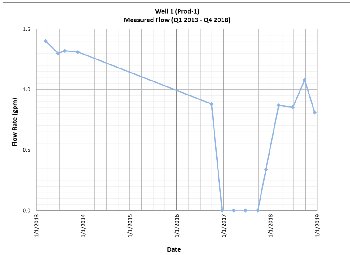
Figure 5. Artesian flows measured at Well 1 (Prod-1)
