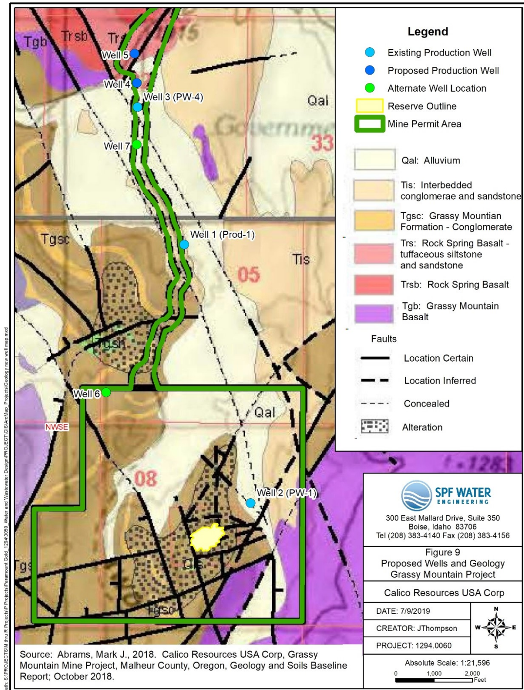
Figure 9. Map of proposed wells and surficial geology
