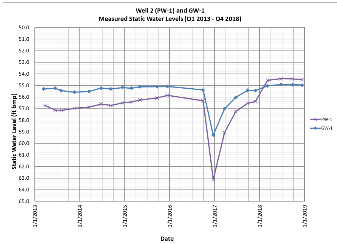
Figure 6. Well 2 (PW-1) and GW-1 static water levels
