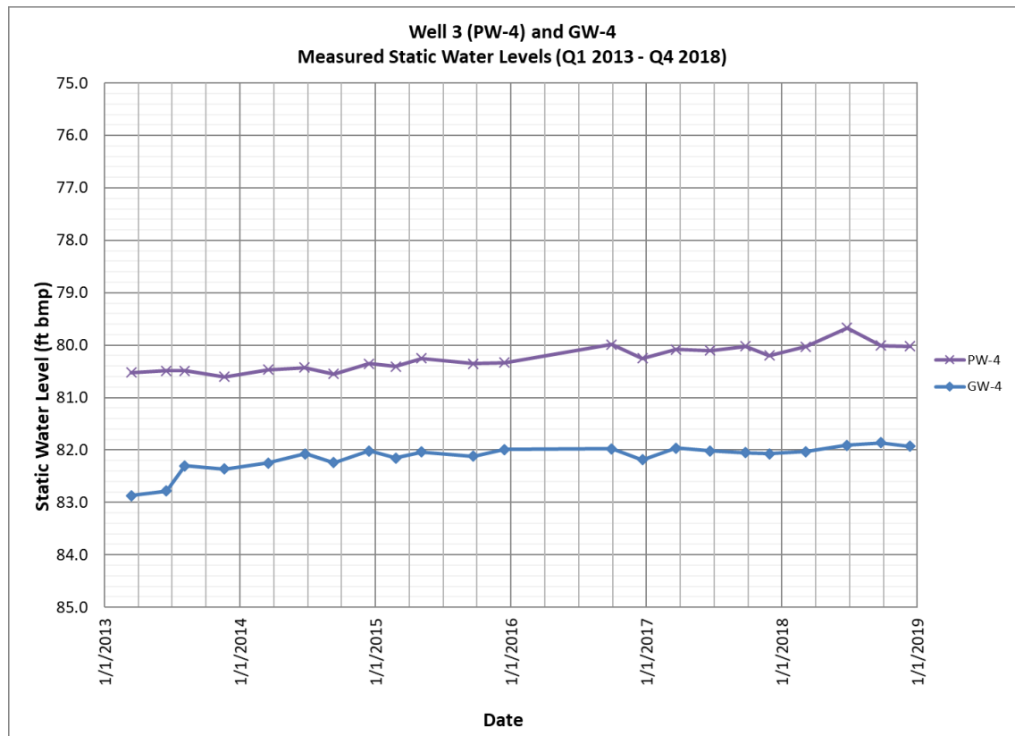
Figure 7. Well 3 (PW-4) and GW-4 static water levels
