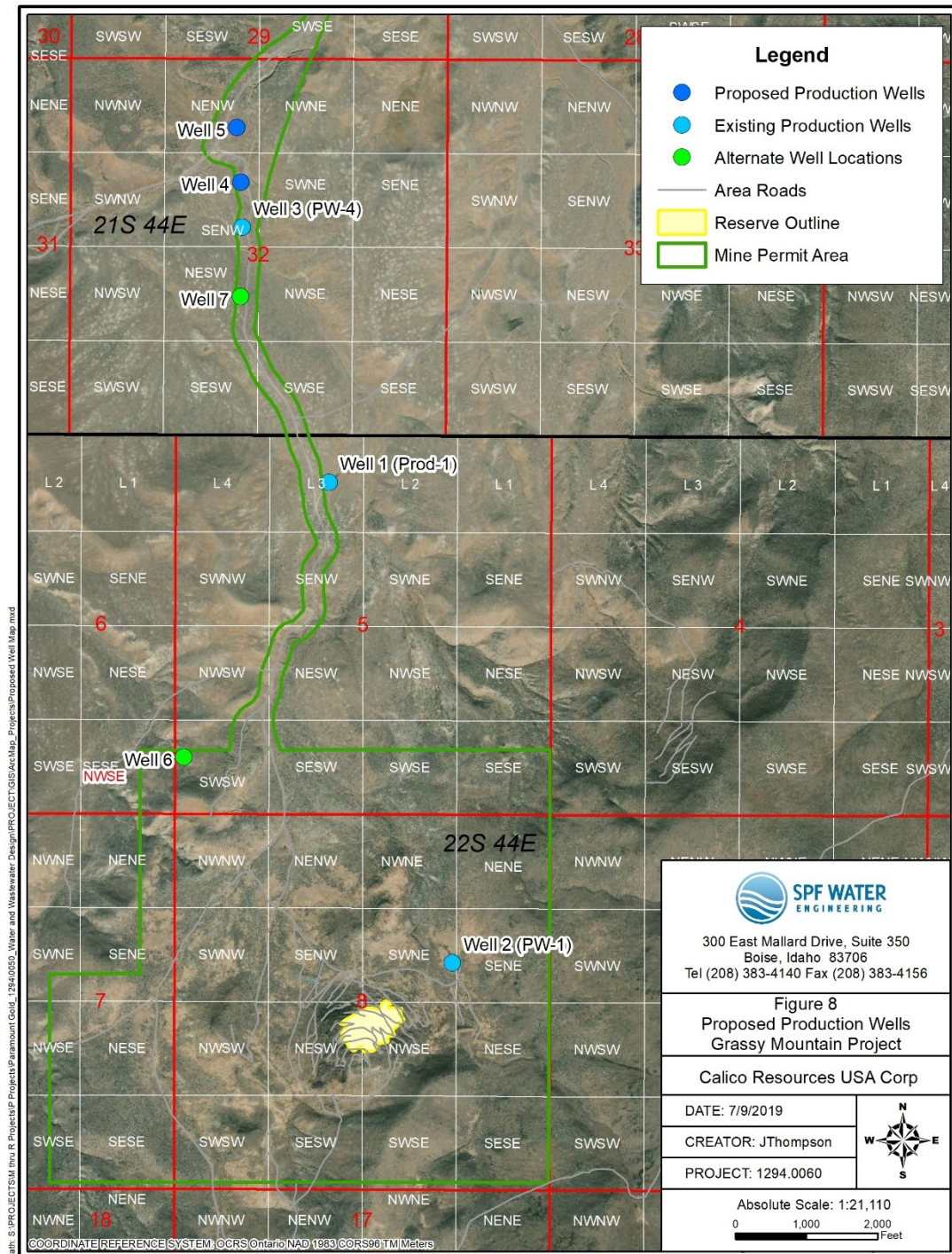
Figure 8. Map of existing and proposed production wells
